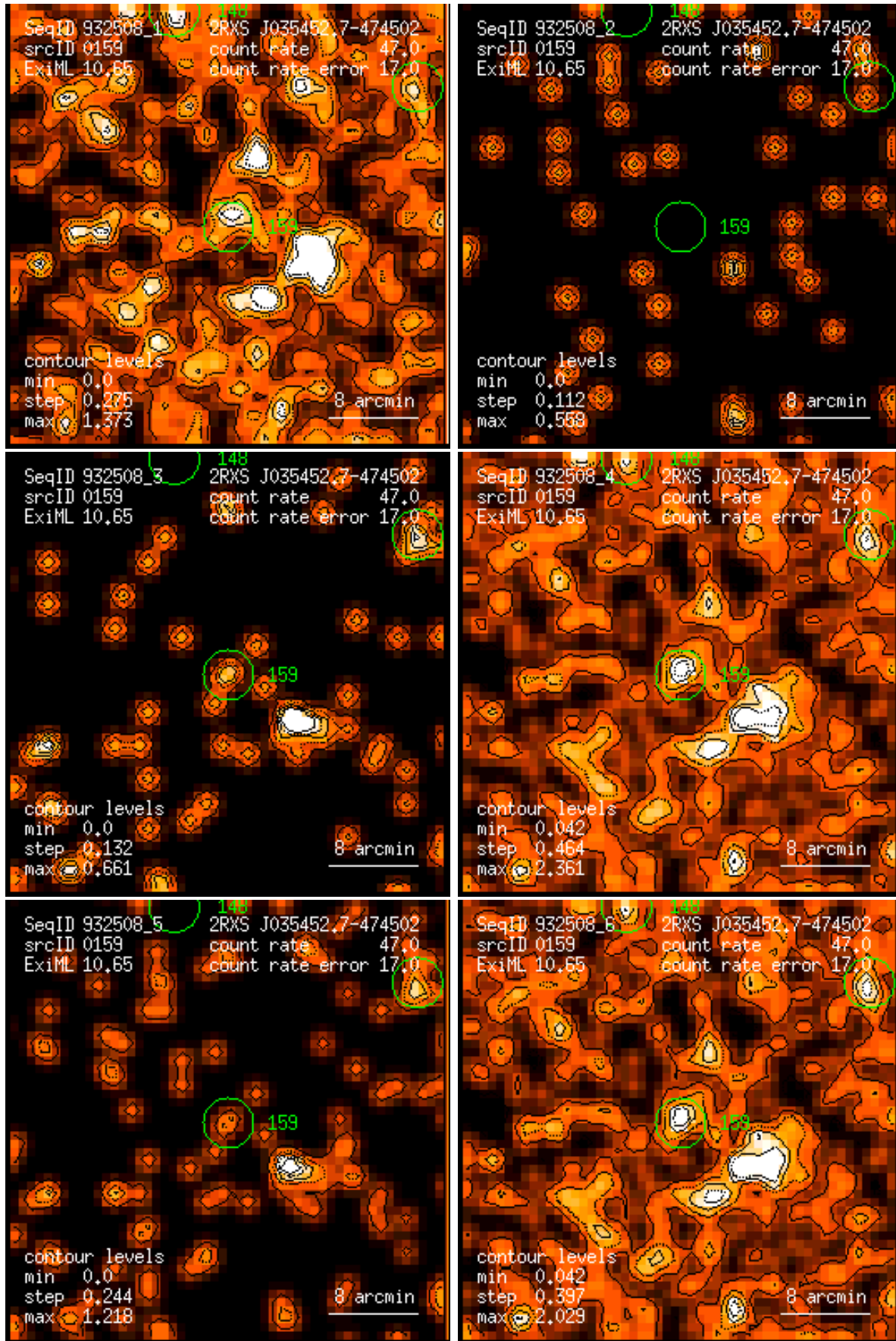
Figure 159: RASS 932508: detection 0159: band rate images, Gaussian filter: (1) PSPC channels 11 – 41, (2) 52 – 90, (3) 91 – 201, (4) 11 – 235, (5) 52 – 201, (6) 11 – 201. Broad band rates in counts/ks. Band rate contour levels in counts/ks/arcmin 2 .
