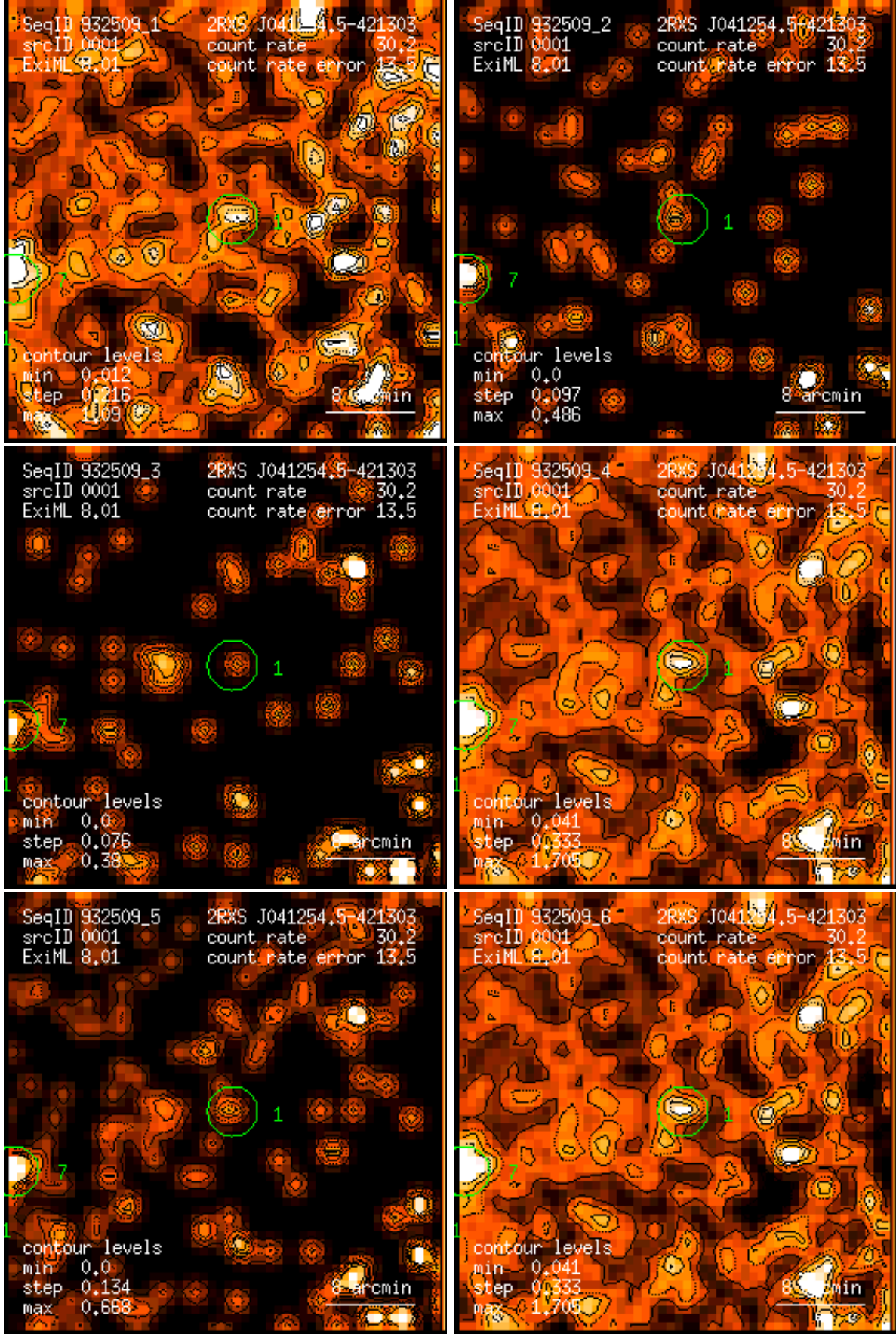
Figure 1: RASS 932509: detection 0001: band rate images, Gaussian filter: (1) PSPC channels 11 – 41, (2) 52 – 90, (3) 91 – 201, (4) 11 – 235, (5) 52 – 201, (6) 11 – 201. Broad band rates in counts/ks. Band rate contour levels in counts/ks/arcmin 2 .
