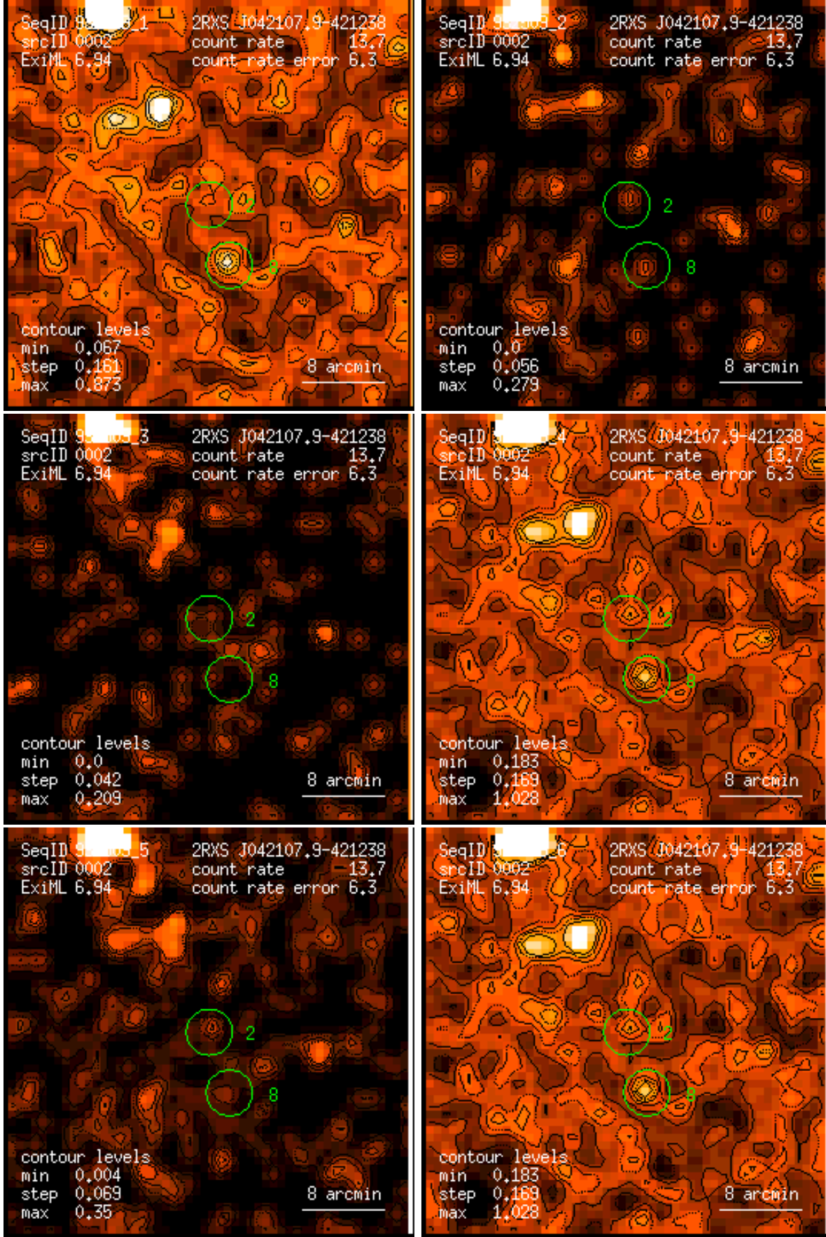
Figure 2: RASS 932509: detection 0002: band rate images, Gaussian filter: (1) PSPC channels 11 – 41, (2) 52 – 90, (3) 91 – 201, (4) 11 – 235, (5) 52 – 201, (6) 11 – 201. Broad band rates in counts/ks. Band rate contour levels in counts/ks/arcmin 2 .
