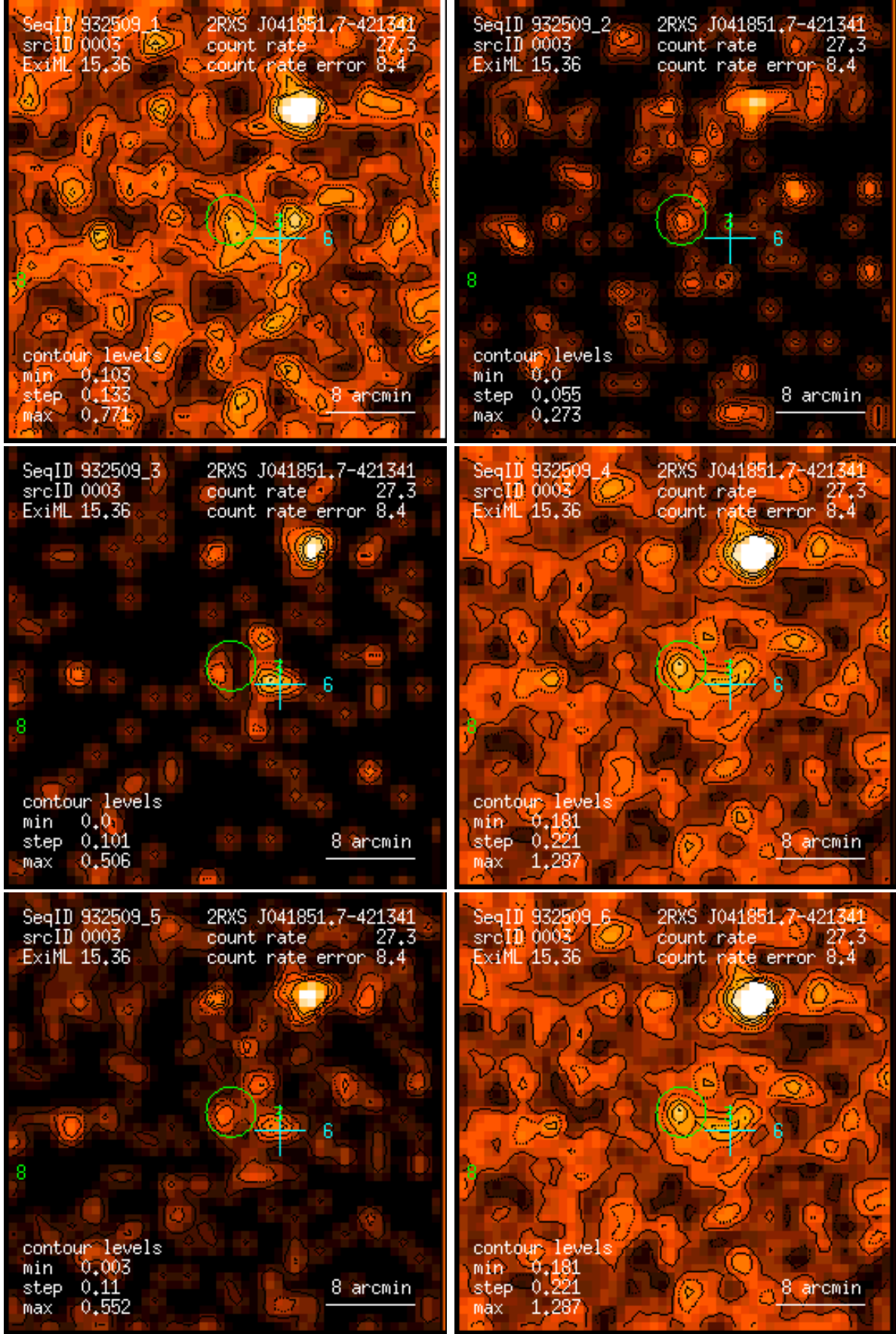
Figure 3: RASS 932509: detection 0003: band rate images, Gaussian filter: (1) PSPC channels 11 – 41, (2) 52 – 90, (3) 91 – 201, (4) 11 – 235, (5) 52 – 201, (6) 11 – 201. Broad band rates in counts/ks. Band rate contour levels in counts/ks/arcmin 2 .
