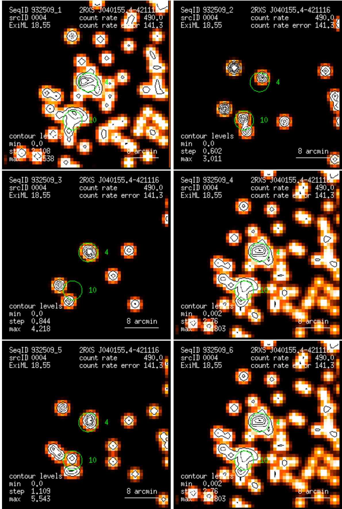
Figure 4: RASS 932509: detection 0004: band rate images, Gaussian filter: (1) PSPC channels 11 – 41, (2) 52 – 90, (3) 91 – 201, (4) 11 – 235, (5) 52 – 201, (6) 11 – 201. Broad band rates in counts/ks. Band rate contour levels in counts/ks/arcmin 2 .
