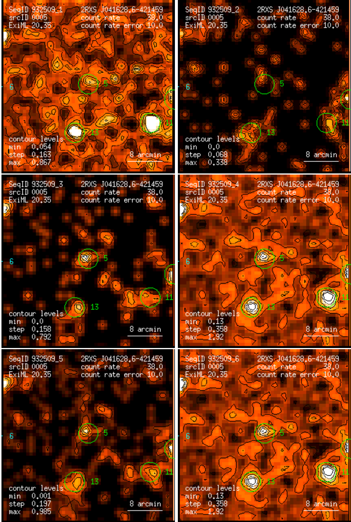
Figure 5: RASS 932509: detection 0005: band rate images, Gaussian filter: (1) PSPC channels 11 – 41, (2) 52 – 90, (3) 91 – 201, (4) 11 – 235, (5) 52 – 201, (6) 11 – 201. Broad band rates in counts/ks. Band rate contour levels in counts/ks/arcmin 2 .
