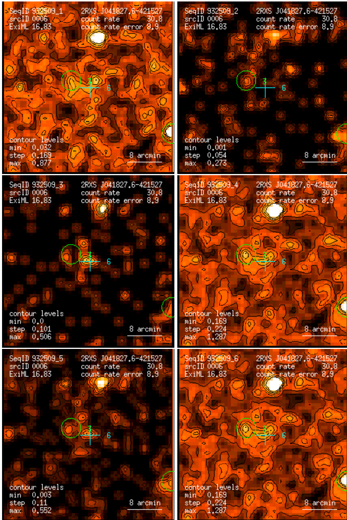
Figure 6: RASS 932509: detection 0006: band rate images, Gaussian filter: (1) PSPC channels 11 – 41, (2) 52 – 90, (3) 91 – 201, (4) 11 – 235, (5) 52 – 201, (6) 11 – 201. Broad band rates in counts/ks. Band rate contour levels in counts/ks/arcmin 2 .
