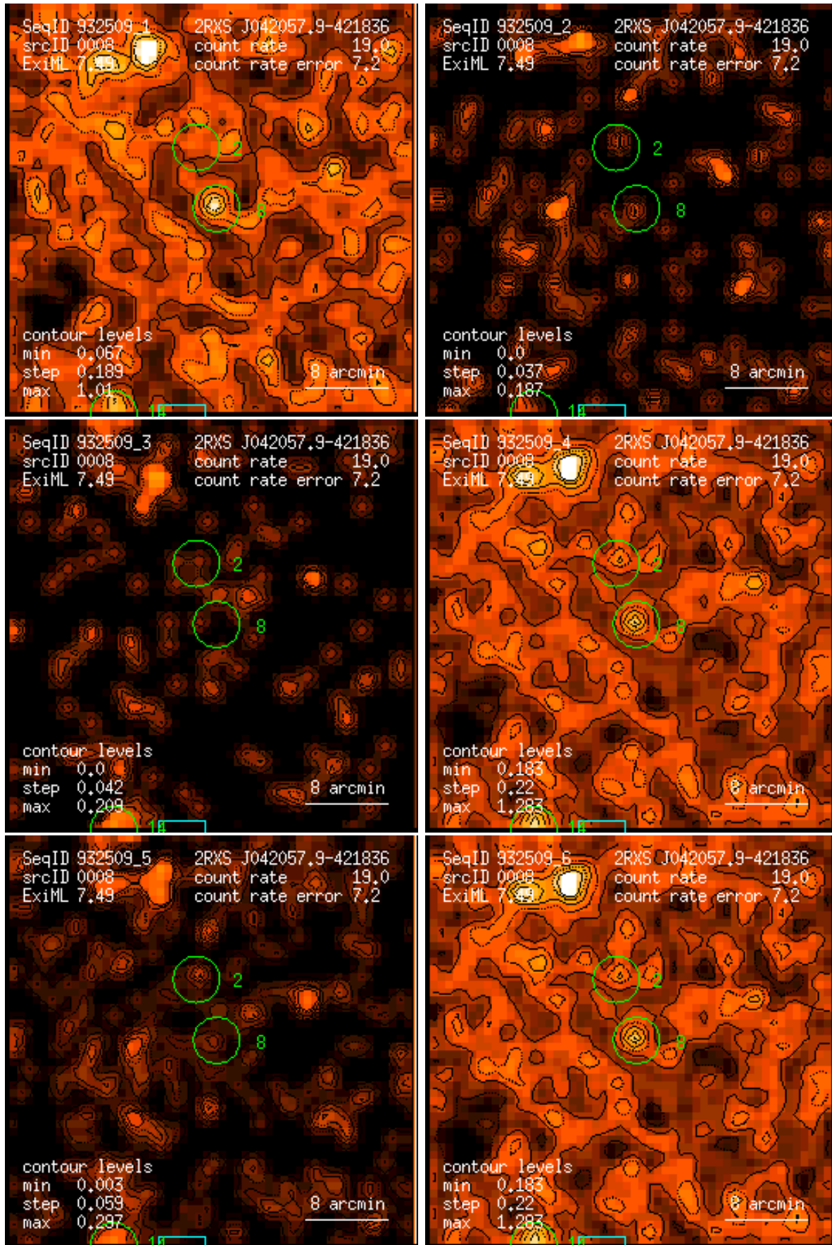
Figure 8: RASS 932509: detection 0008: band rate images, Gaussian filter: (1) PSPC channels 11 – 41, (2) 52 – 90, (3) 91 – 201, (4) 11 – 235, (5) 52 – 201, (6) 11 – 201. Broad band rates in counts/ks. Band rate contour levels in counts/ks/arcmin 2 .
