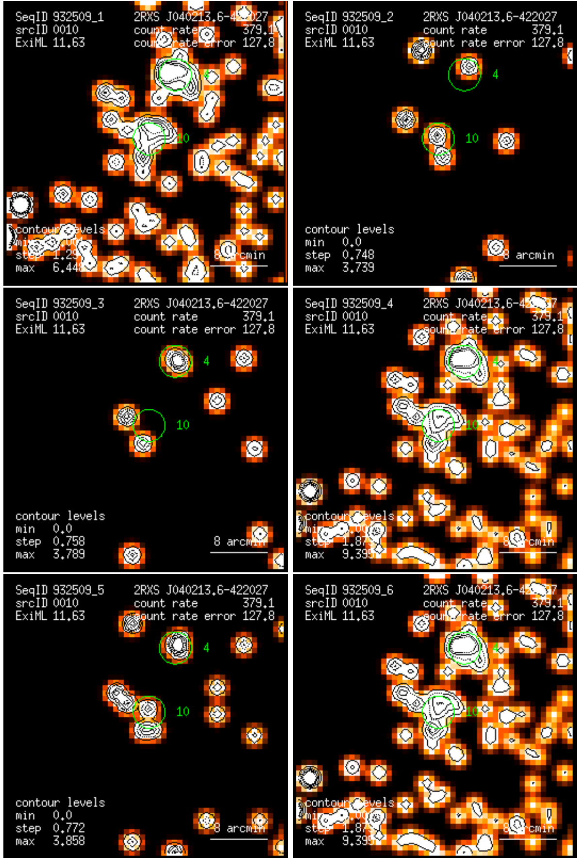
Figure 10: RASS 932509: detection 0010: band rate images, Gaussian filter: (1) PSPC channels 11 – 41, (2) 52 – 90, (3) 91 – 201, (4) 11 – 235, (5) 52 – 201, (6) 11 – 201. Broad band rates in counts/ks. Band rate contour levels in counts/ks/arcmin 2 .
