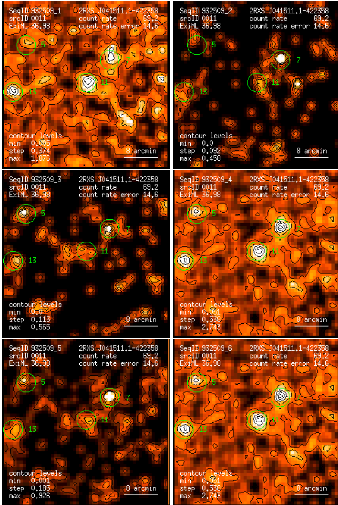
Figure 11: RASS 932509: detection 0011: band rate images, Gaussian filter: (1) PSPC channels 11 – 41, (2) 52 – 90, (3) 91 – 201, (4) 11 – 235, (5) 52 – 201, (6) 11 – 201. Broad band rates in counts/ks. Band rate contour levels in counts/ks/arcmin 2 .
