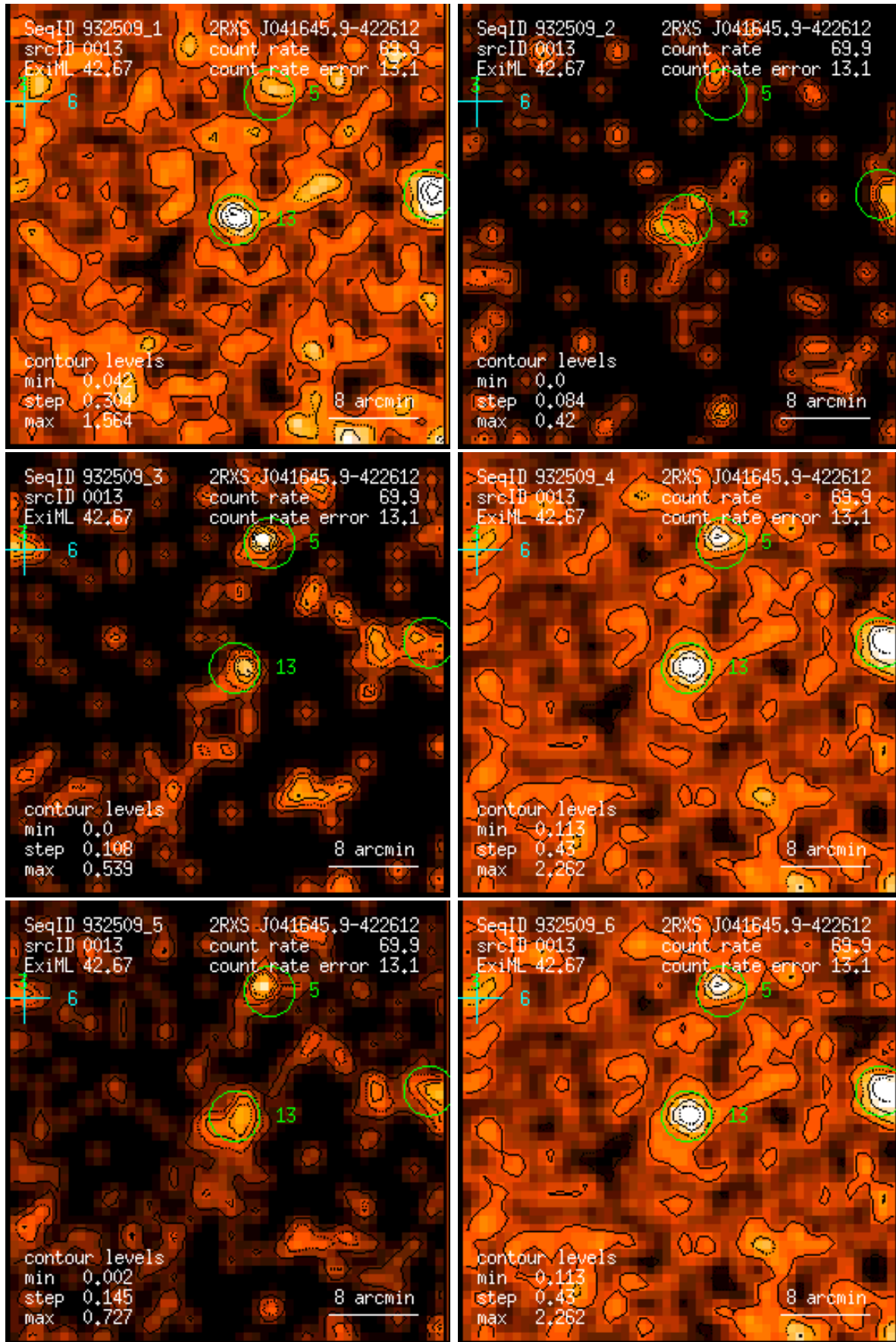
Figure 13: RASS 932509: detection 0013: band rate images, Gaussian filter: (1) PSPC channels 11 – 41, (2) 52 – 90, (3) 91 – 201, (4) 11 – 235, (5) 52 – 201, (6) 11 – 201. Broad band rates in counts/ks. Band rate contour levels in counts/ks/arcmin 2 .
