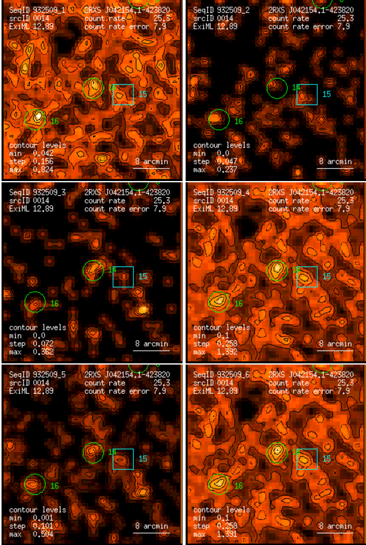
Figure 14: RASS 932509: detection 0014: band rate images, Gaussian filter: (1) PSPC channels 11 – 41, (2) 52 – 90, (3) 91 – 201, (4) 11 – 235, (5) 52 – 201, (6) 11 – 201. Broad band rates in counts/ks. Band rate contour levels in counts/ks/arcmin 2 .
