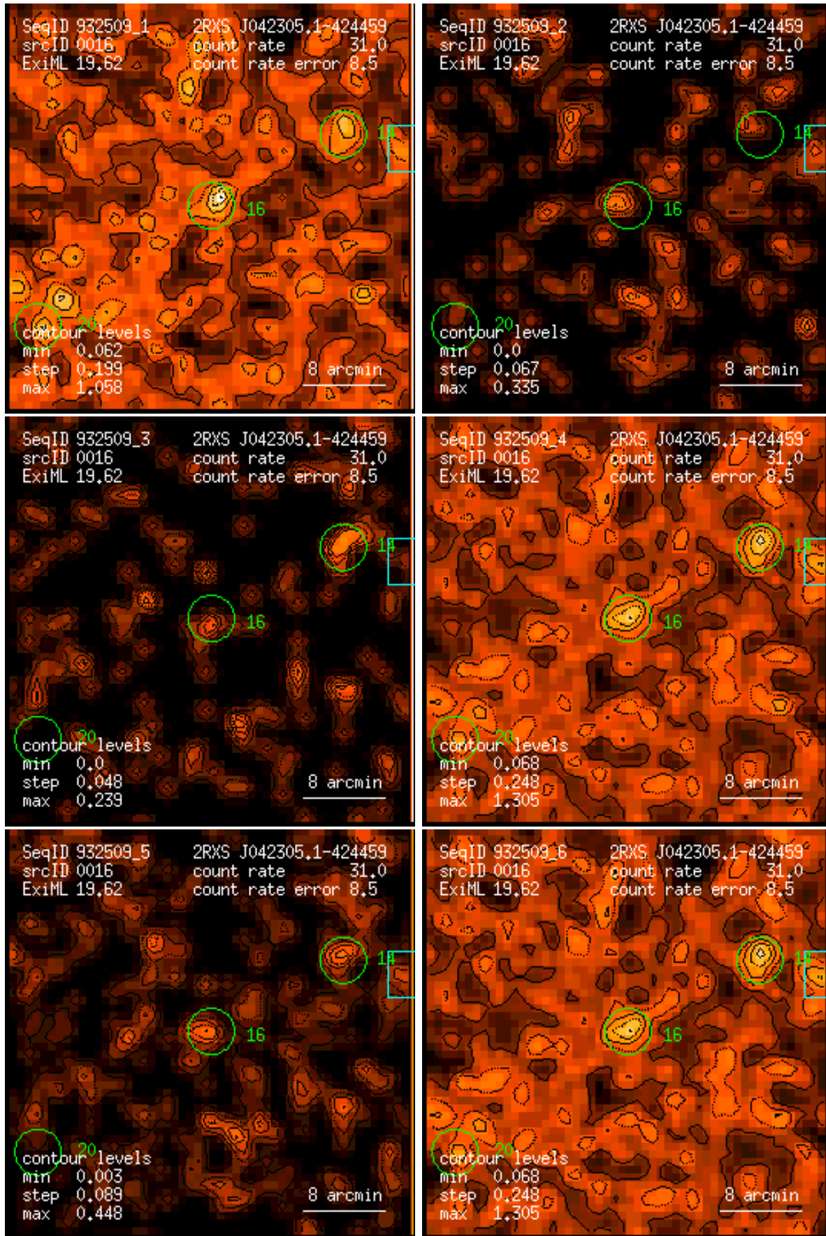
Figure 16: RASS 932509: detection 0016: band rate images, Gaussian filter: (1) PSPC channels 11 – 41, (2) 52 – 90, (3) 91 – 201, (4) 11 – 235, (5) 52 – 201, (6) 11 – 201. Broad band rates in counts/ks. Band rate contour levels in counts/ks/arcmin 2 .
