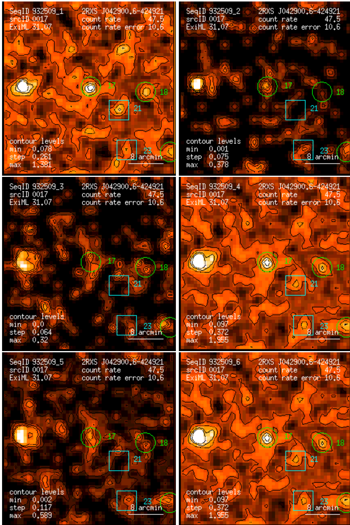
Figure 17: RASS 932509: detection 0017: band rate images, Gaussian filter: (1) PSPC channels 11 – 41, (2) 52 – 90, (3) 91 – 201, (4) 11 – 235, (5) 52 – 201, (6) 11 – 201. Broad band rates in counts/ks. Band rate contour levels in counts/ks/arcmin 2 .
