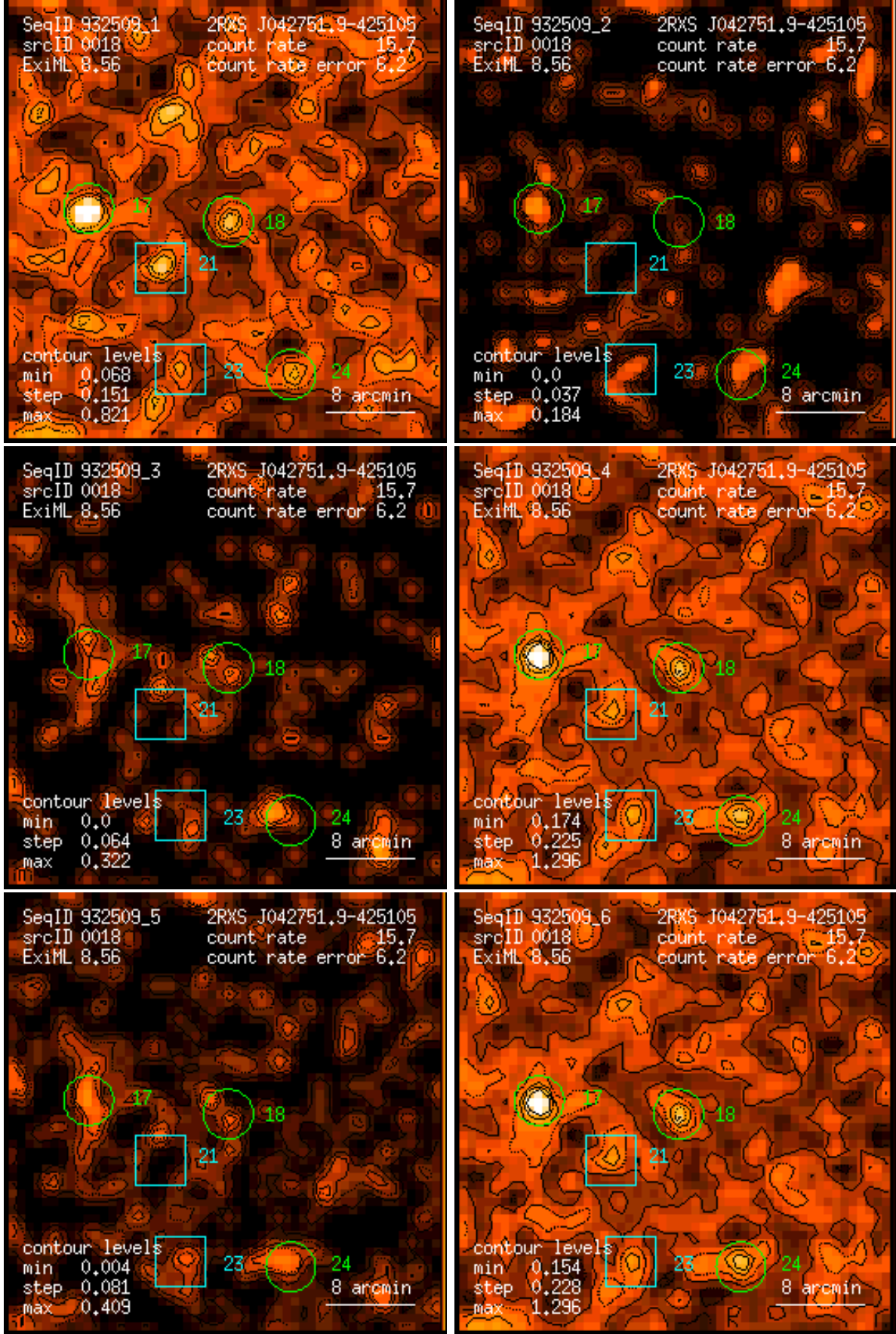
Figure 18: RASS 932509: detection 0018: band rate images, Gaussian filter: (1) PSPC channels 11 – 41, (2) 52 – 90, (3) 91 – 201, (4) 11 – 235, (5) 52 – 201, (6) 11 – 201. Broad band rates in counts/ks. Band rate contour levels in counts/ks/arcmin 2 .
