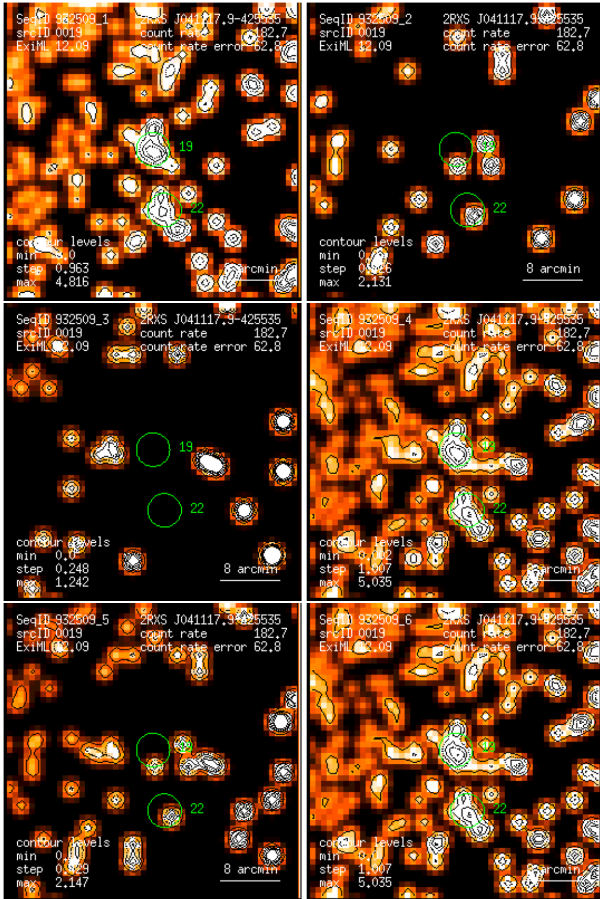
Figure 19: RASS 932509: detection 0019: band rate images, Gaussian filter: (1) PSPC channels 11 – 41, (2) 52 – 90, (3) 91 – 201, (4) 11 – 235, (5) 52 – 201, (6) 11 – 201. Broad band rates in counts/ks. Band rate contour levels in counts/ks/arcmin 2 .
