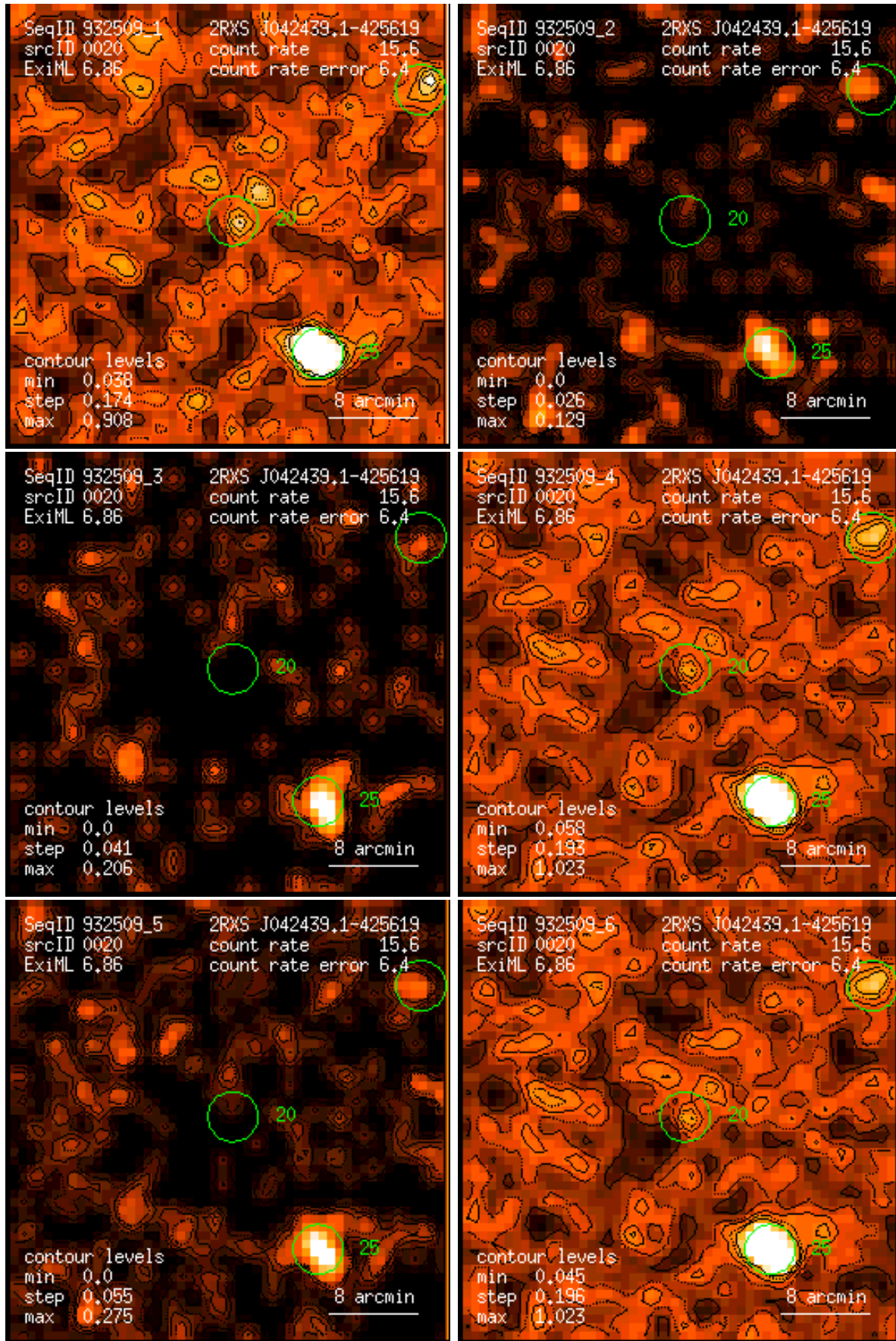
Figure 20: RASS 932509: detection 0020: band rate images, Gaussian filter: (1) PSPC channels 11 – 41, (2) 52 – 90, (3) 91 – 201, (4) 11 – 235, (5) 52 – 201, (6) 11 – 201. Broad band rates in counts/ks. Band rate contour levels in counts/ks/arcmin 2 .
