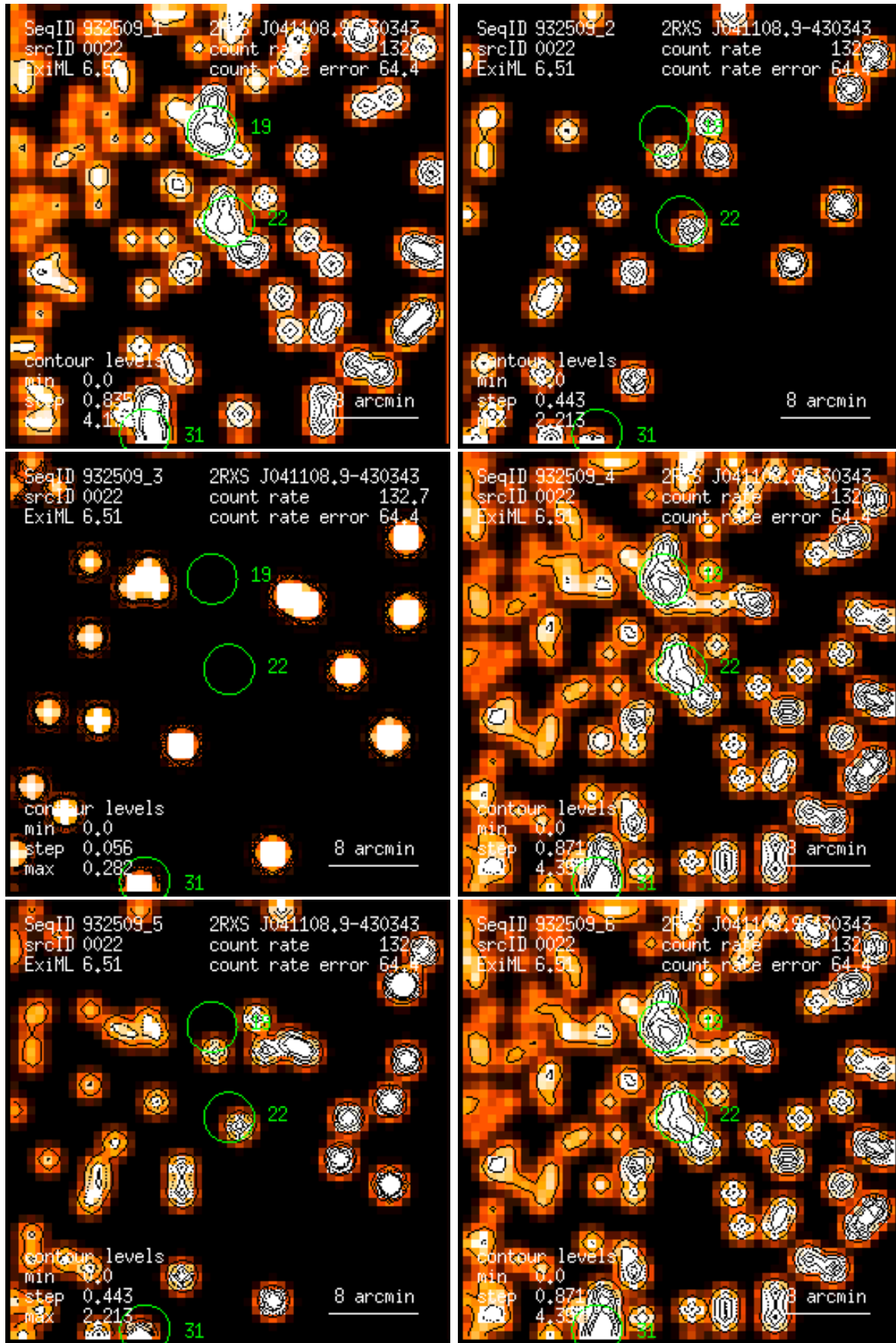
Figure 22: RASS 932509: detection 0022: band rate images, Gaussian filter: (1) PSPC channels 11 – 41, (2) 52 – 90, (3) 91 – 201, (4) 11 – 235, (5) 52 – 201, (6) 11 – 201. Broad band rates in counts/ks. Band rate contour levels in counts/ks/arcmin 2 .
