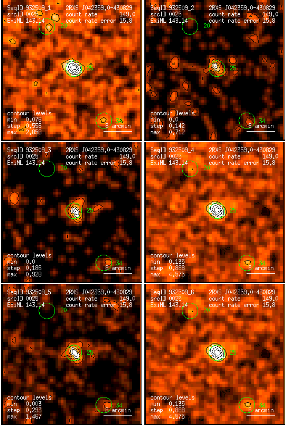
Figure 25: RASS 932509: detection 0025: band rate images, Gaussian filter: (1) PSPC channels 11 – 41, (2) 52 – 90, (3) 91 – 201, (4) 11 – 235, (5) 52 – 201, (6) 11 – 201. Broad band rates in counts/ks. Band rate contour levels in counts/ks/arcmin 2 .
