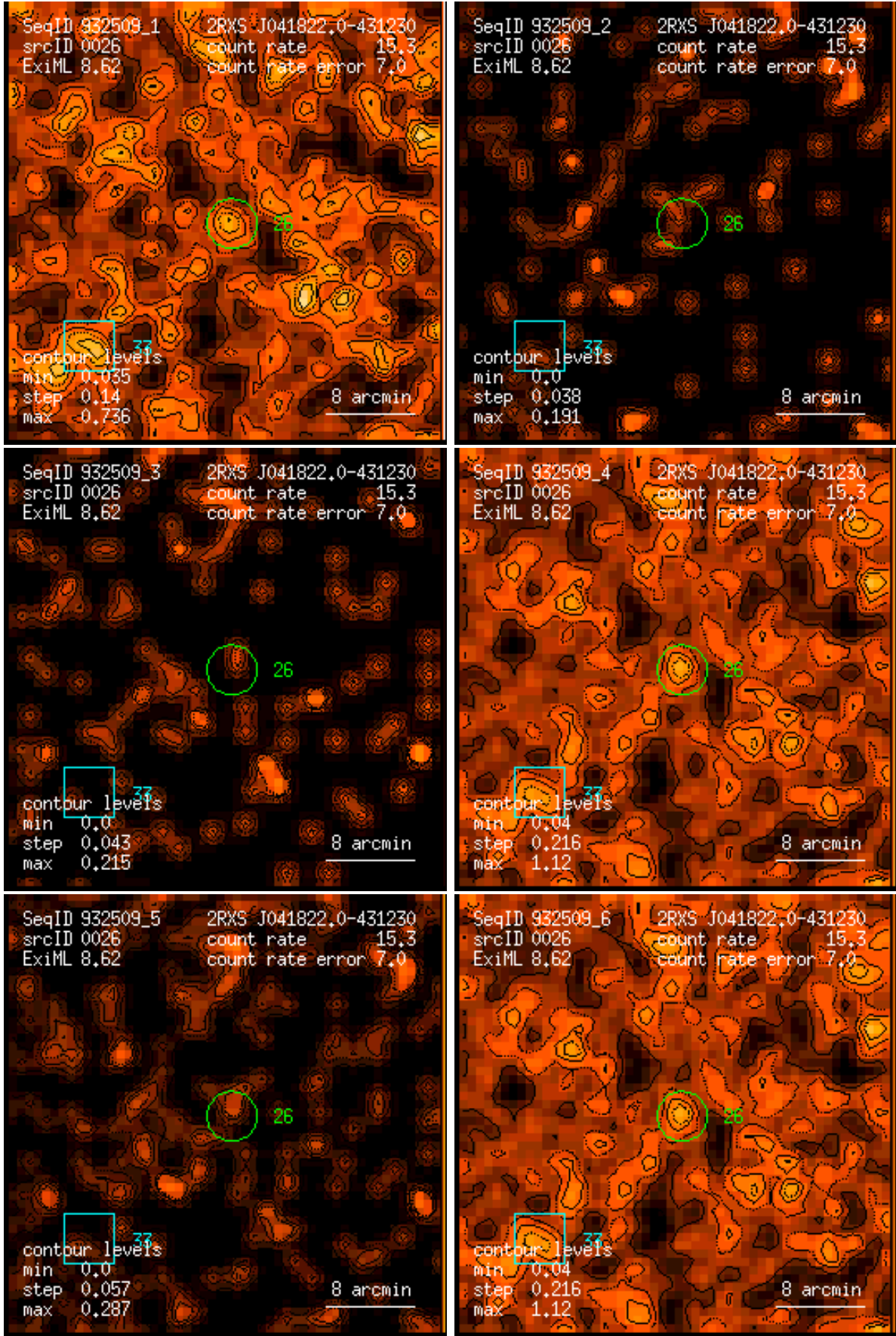
Figure 26: RASS 932509: detection 0026: band rate images, Gaussian filter: (1) PSPC channels 11 – 41, (2) 52 – 90, (3) 91 – 201, (4) 11 – 235, (5) 52 – 201, (6) 11 – 201. Broad band rates in counts/ks. Band rate contour levels in counts/ks/arcmin 2 .
