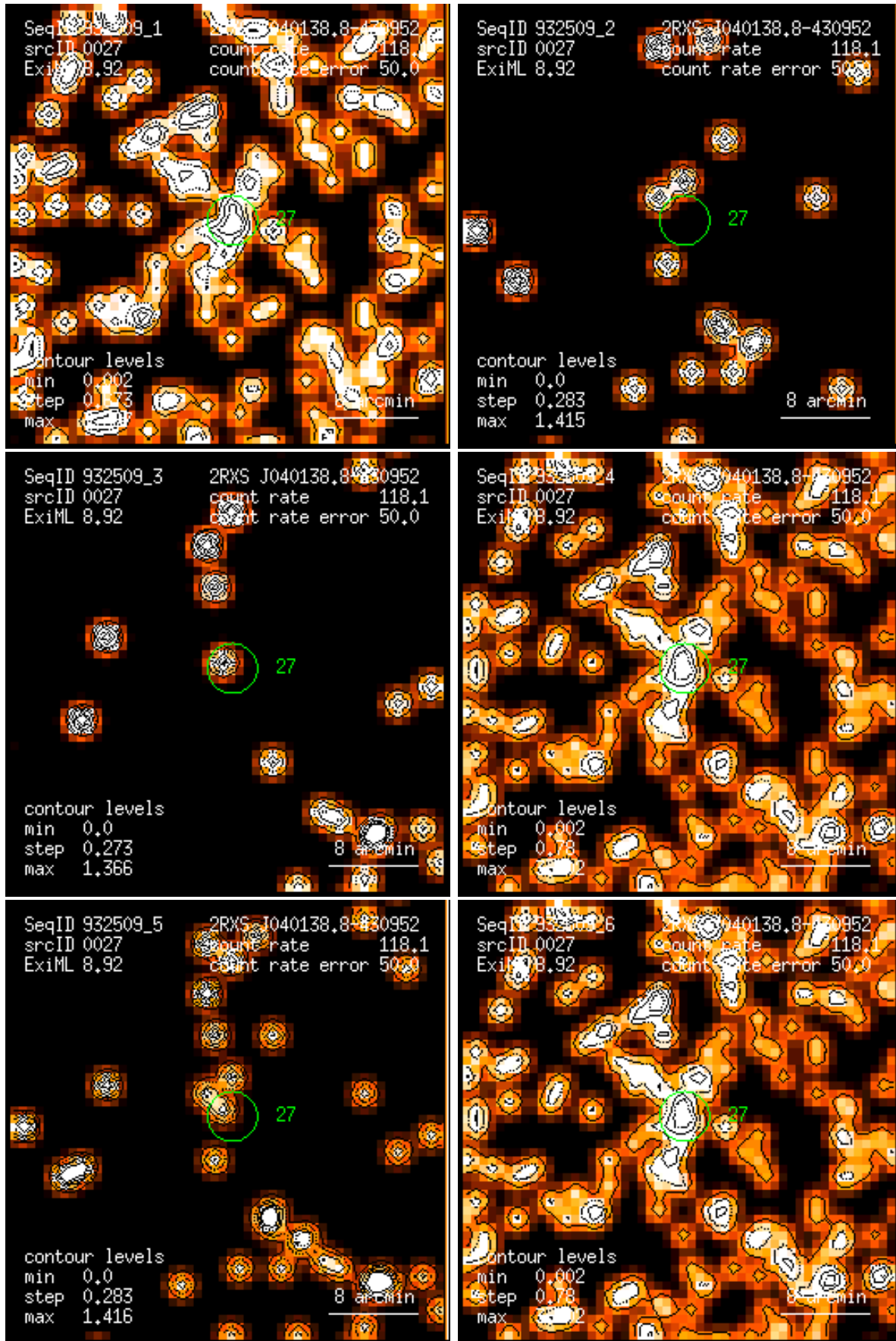
Figure 27: RASS 932509: detection 0027: band rate images, Gaussian filter: (1) PSPC channels 11 – 41, (2) 52 – 90, (3) 91 – 201, (4) 11 – 235, (5) 52 – 201, (6) 11 – 201. Broad band rates in counts/ks. Band rate contour levels in counts/ks/arcmin 2 .
