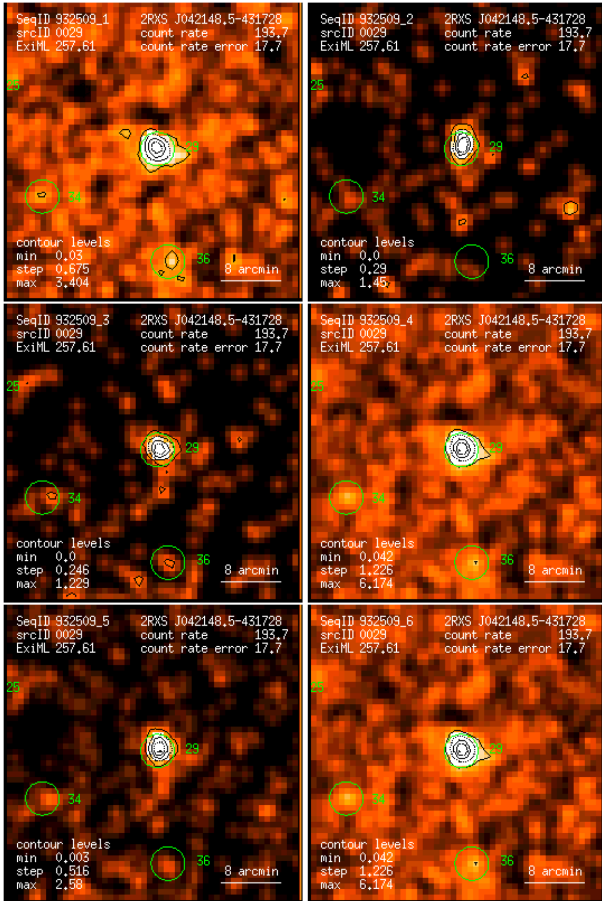
Figure 29: RASS 932509: detection 0029: band rate images, Gaussian filter: (1) PSPC channels 11 – 41, (2) 52 – 90, (3) 91 – 201, (4) 11 – 235, (5) 52 – 201, (6) 11 – 201. Broad band rates in counts/ks. Band rate contour levels in counts/ks/arcmin 2 .
