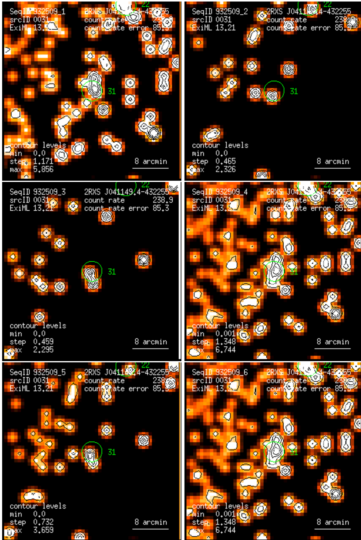
Figure 31: RASS 932509: detection 0031: band rate images, Gaussian filter: (1) PSPC channels 11 – 41, (2) 52 – 90, (3) 91 – 201, (4) 11 – 235, (5) 52 – 201, (6) 11 – 201. Broad band rates in counts/ks. Band rate contour levels in counts/ks/arcmin 2 .
