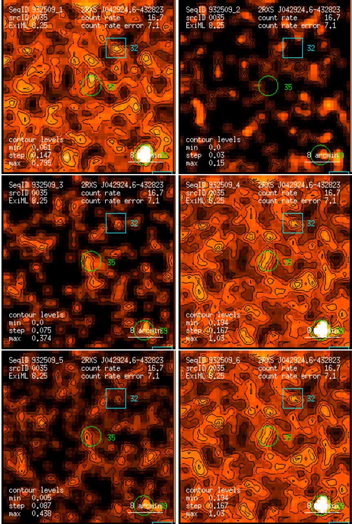
Figure 35: RASS 932509: detection 0035: band rate images, Gaussian filter: (1) PSPC channels 11 – 41, (2) 52 – 90, (3) 91 – 201, (4) 11 – 235, (5) 52 – 201, (6) 11 – 201. Broad band rates in counts/ks. Band rate contour levels in counts/ks/arcmin 2 .
