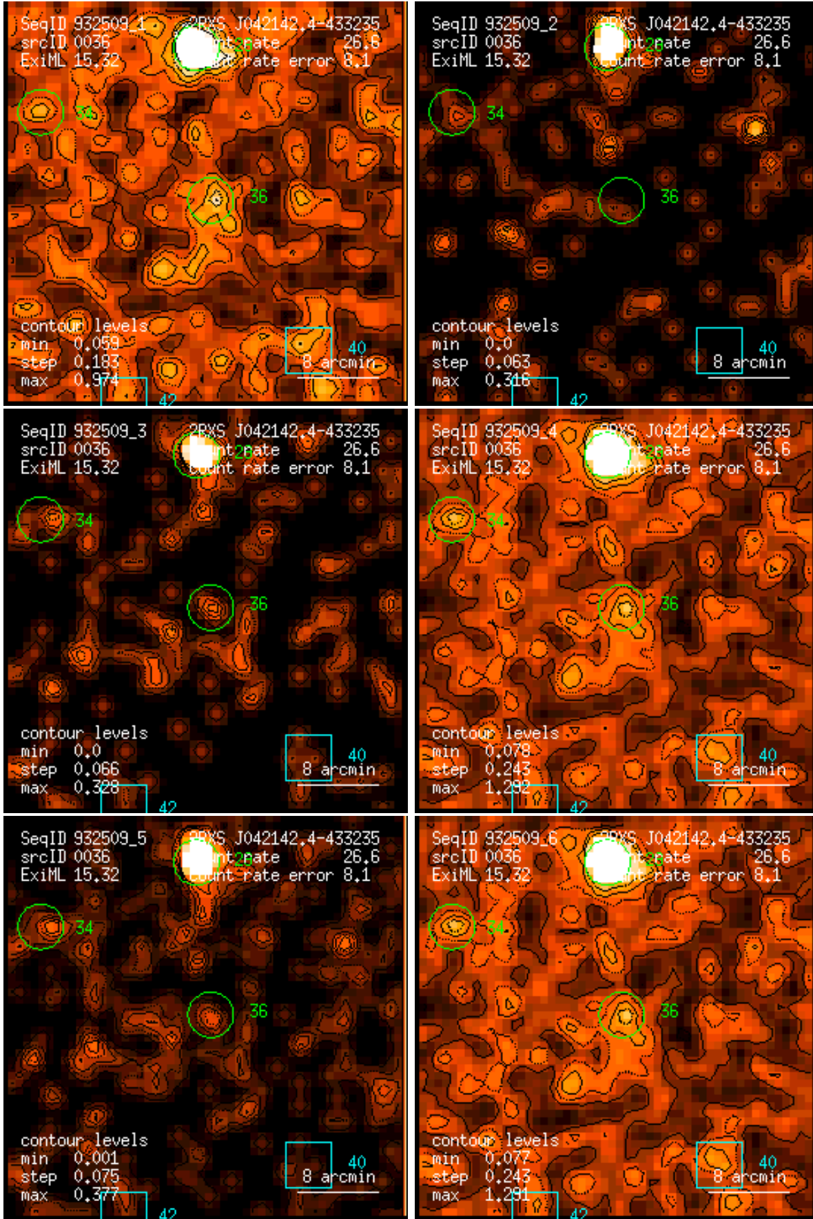
Figure 36: RASS 932509: detection 0036: band rate images, Gaussian filter: (1) PSPC channels 11 – 41, (2) 52 – 90, (3) 91 – 201, (4) 11 – 235, (5) 52 – 201, (6) 11 – 201. Broad band rates in counts/ks. Band rate contour levels in counts/ks/arcmin 2 .
