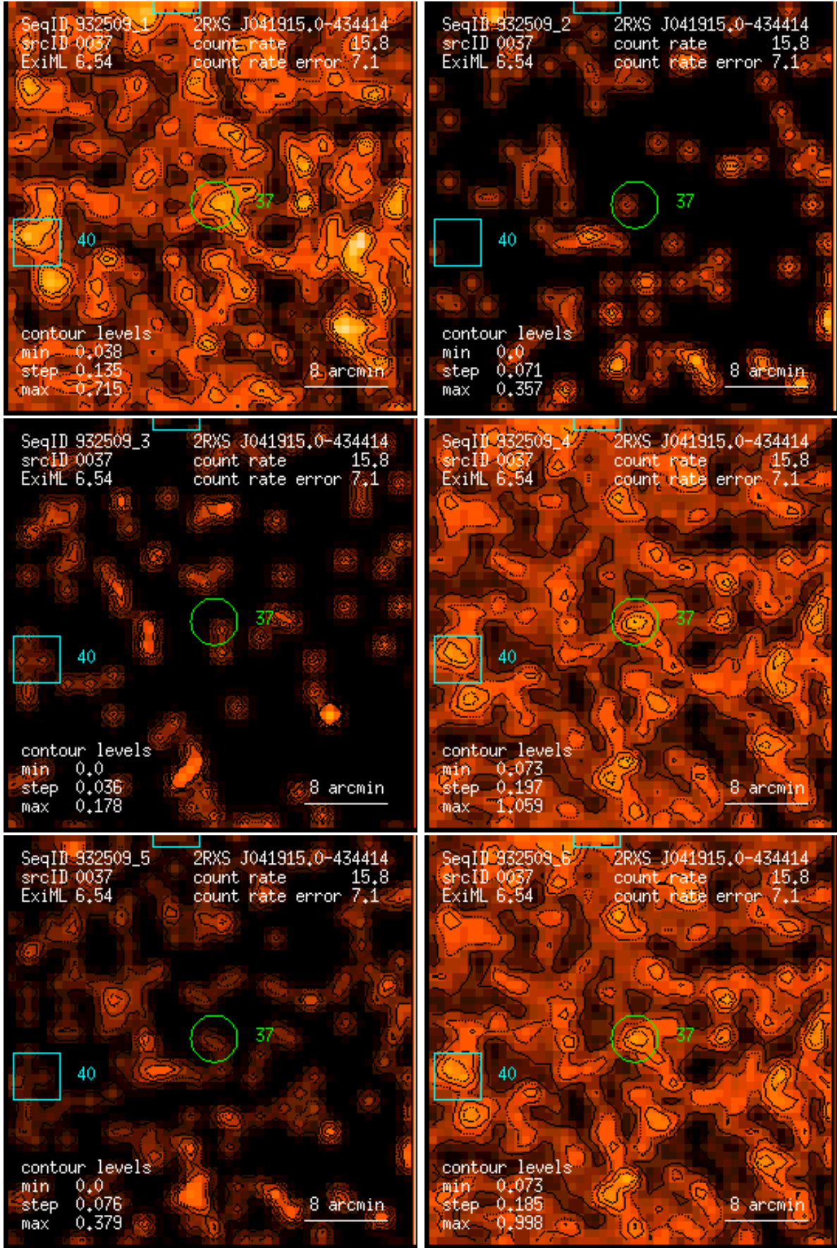
Figure 37: RASS 932509: detection 0037: band rate images, Gaussian filter: (1) PSPC channels 11 – 41, (2) 52 – 90, (3) 91 – 201, (4) 11 – 235, (5) 52 – 201, (6) 11 – 201. Broad band rates in counts/ks. Band rate contour levels in counts/ks/arcmin 2 .
