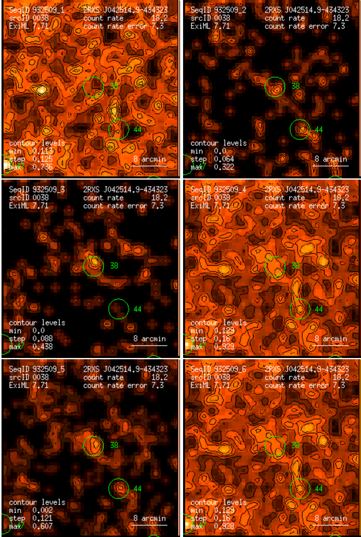
Figure 38: RASS 932509: detection 0038: band rate images, Gaussian filter: (1) PSPC channels 11 – 41, (2) 52 – 90, (3) 91 – 201, (4) 11 – 235, (5) 52 – 201, (6) 11 – 201. Broad band rates in counts/ks. Band rate contour levels in counts/ks/arcmin 2 .
