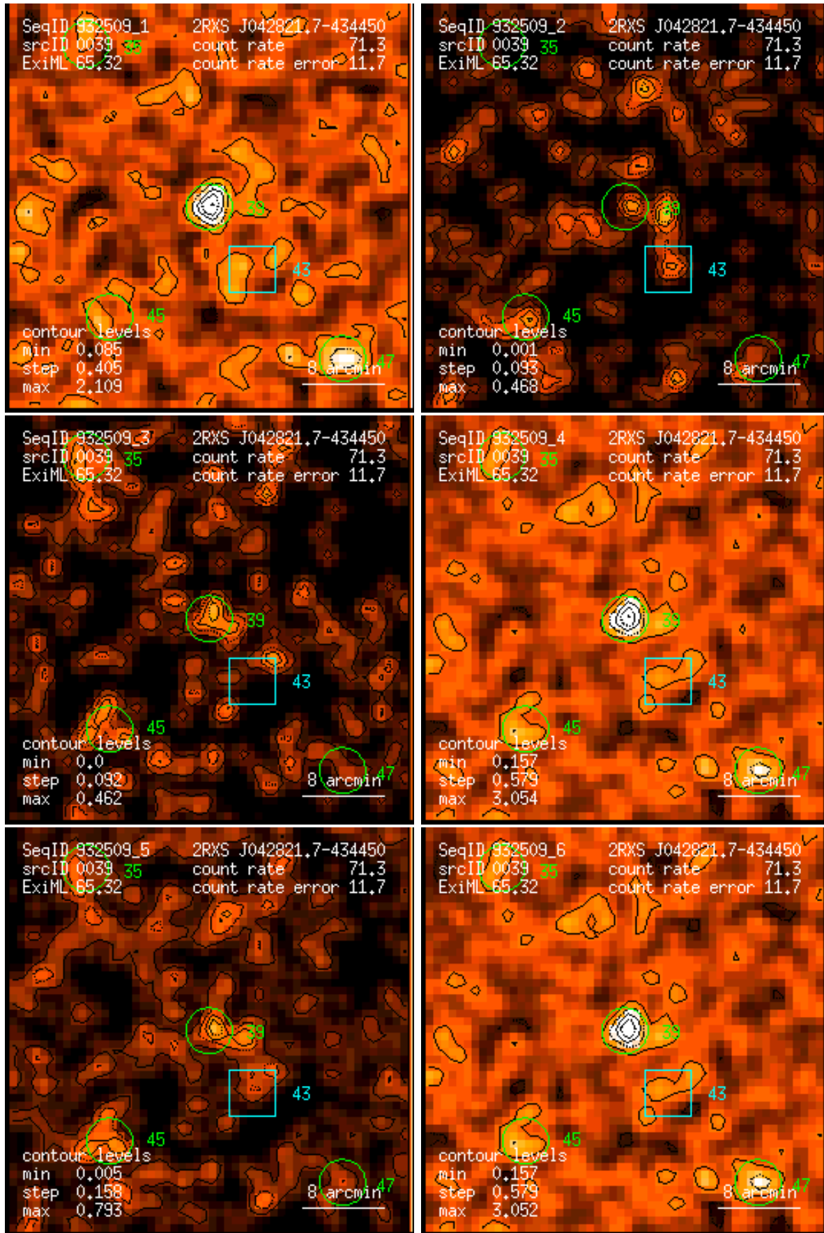
Figure 39: RASS 932509: detection 0039: band rate images, Gaussian filter: (1) PSPC channels 11 – 41, (2) 52 – 90, (3) 91 – 201, (4) 11 – 235, (5) 52 – 201, (6) 11 – 201. Broad band rates in counts/ks. Band rate contour levels in counts/ks/arcmin 2 .
