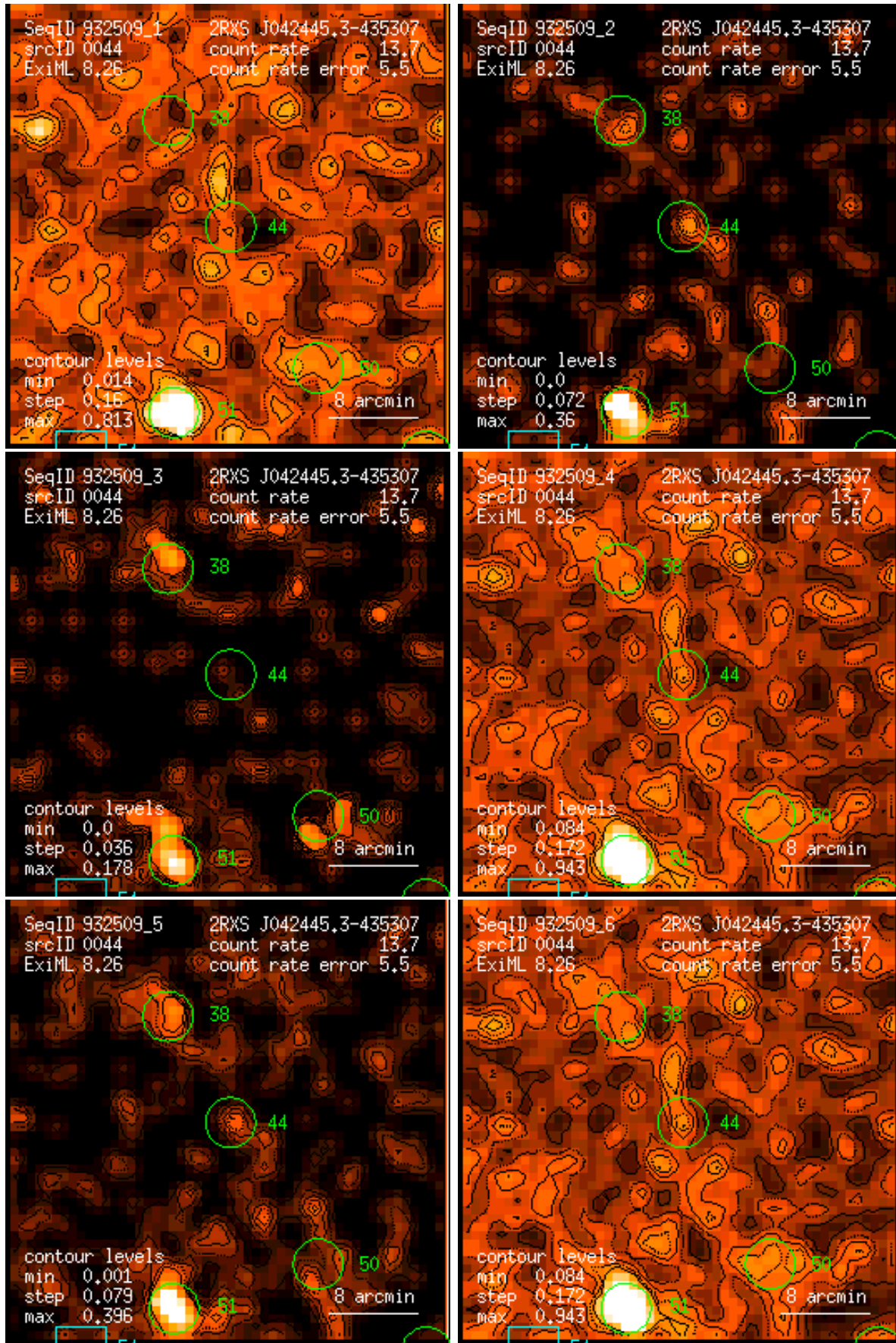
Figure 44: RASS 932509: detection 0044: band rate images, Gaussian filter: (1) PSPC channels 11 – 41, (2) 52 – 90, (3) 91 – 201, (4) 11 – 235, (5) 52 – 201, (6) 11 – 201. Broad band rates in counts/ks. Band rate contour levels in counts/ks/arcmin 2 .
