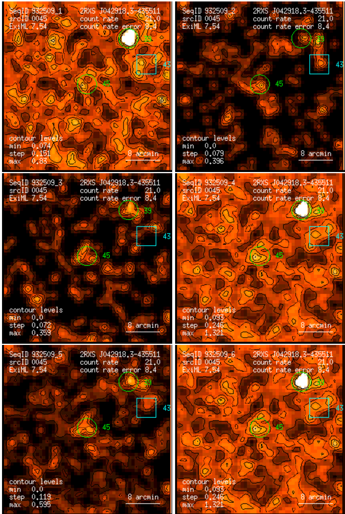
Figure 45: RASS 932509: detection 0045: band rate images, Gaussian filter: (1) PSPC channels 11 – 41, (2) 52 – 90, (3) 91 – 201, (4) 11 – 235, (5) 52 – 201, (6) 11 – 201. Broad band rates in counts/ks. Band rate contour levels in counts/ks/arcmin 2 .
