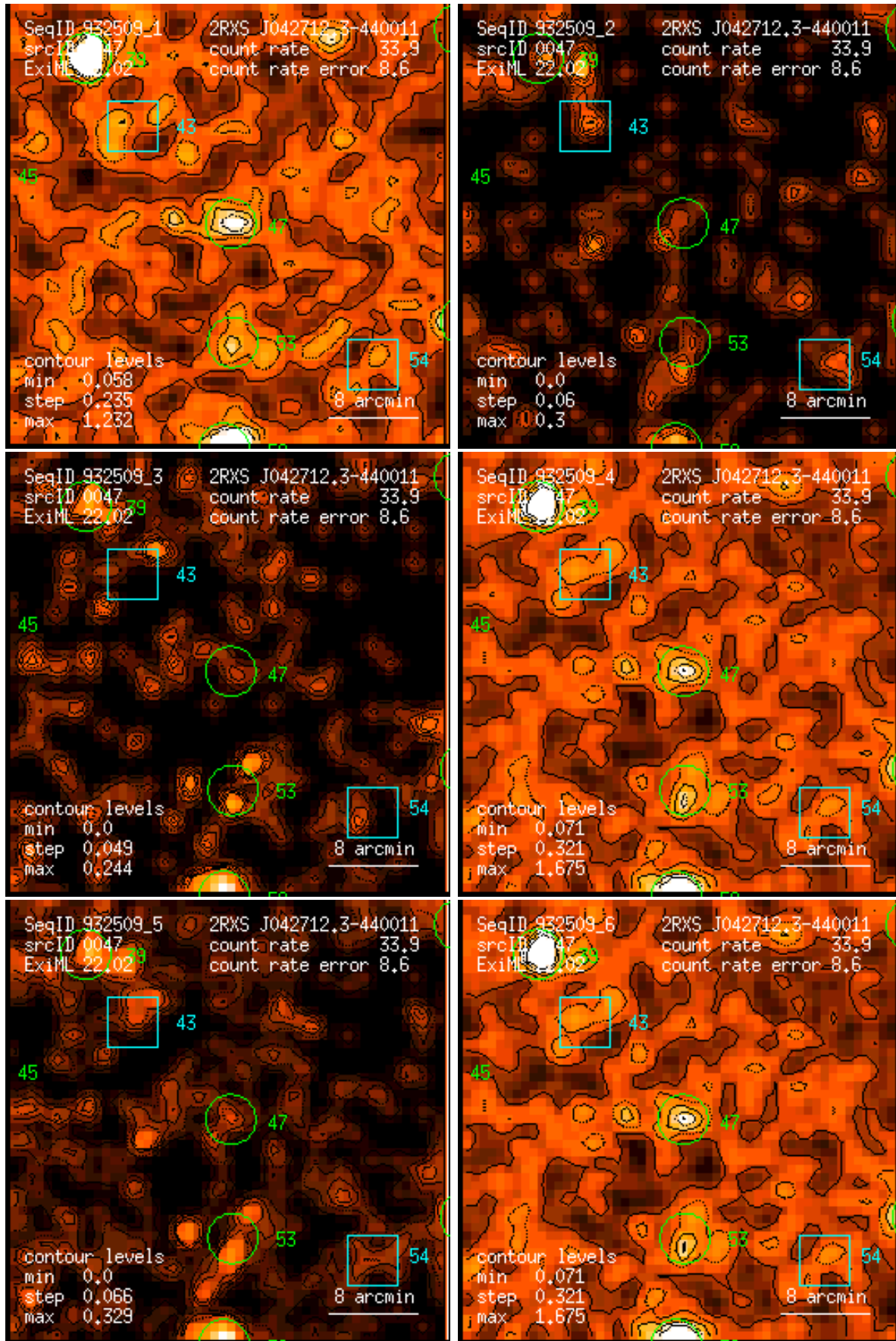
Figure 47: RASS 932509: detection 0047: band rate images, Gaussian filter: (1) PSPC channels 11 – 41, (2) 52 – 90, (3) 91 – 201, (4) 11 – 235, (5) 52 – 201, (6) 11 – 201. Broad band rates in counts/ks. Band rate contour levels in counts/ks/arcmin 2 .
