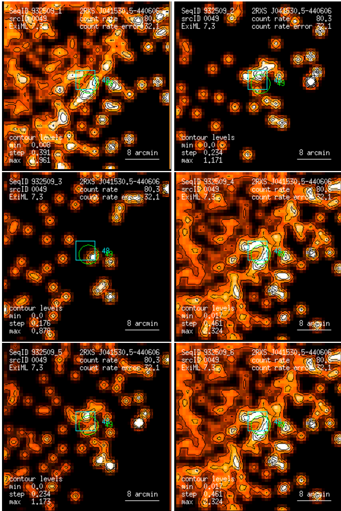
Figure 49: RASS 932509: detection 0049: band rate images, Gaussian filter: (1) PSPC channels 11 – 41, (2) 52 – 90, (3) 91 – 201, (4) 11 – 235, (5) 52 – 201, (6) 11 – 201. Broad band rates in counts/ks. Band rate contour levels in counts/ks/arcmin 2 .
