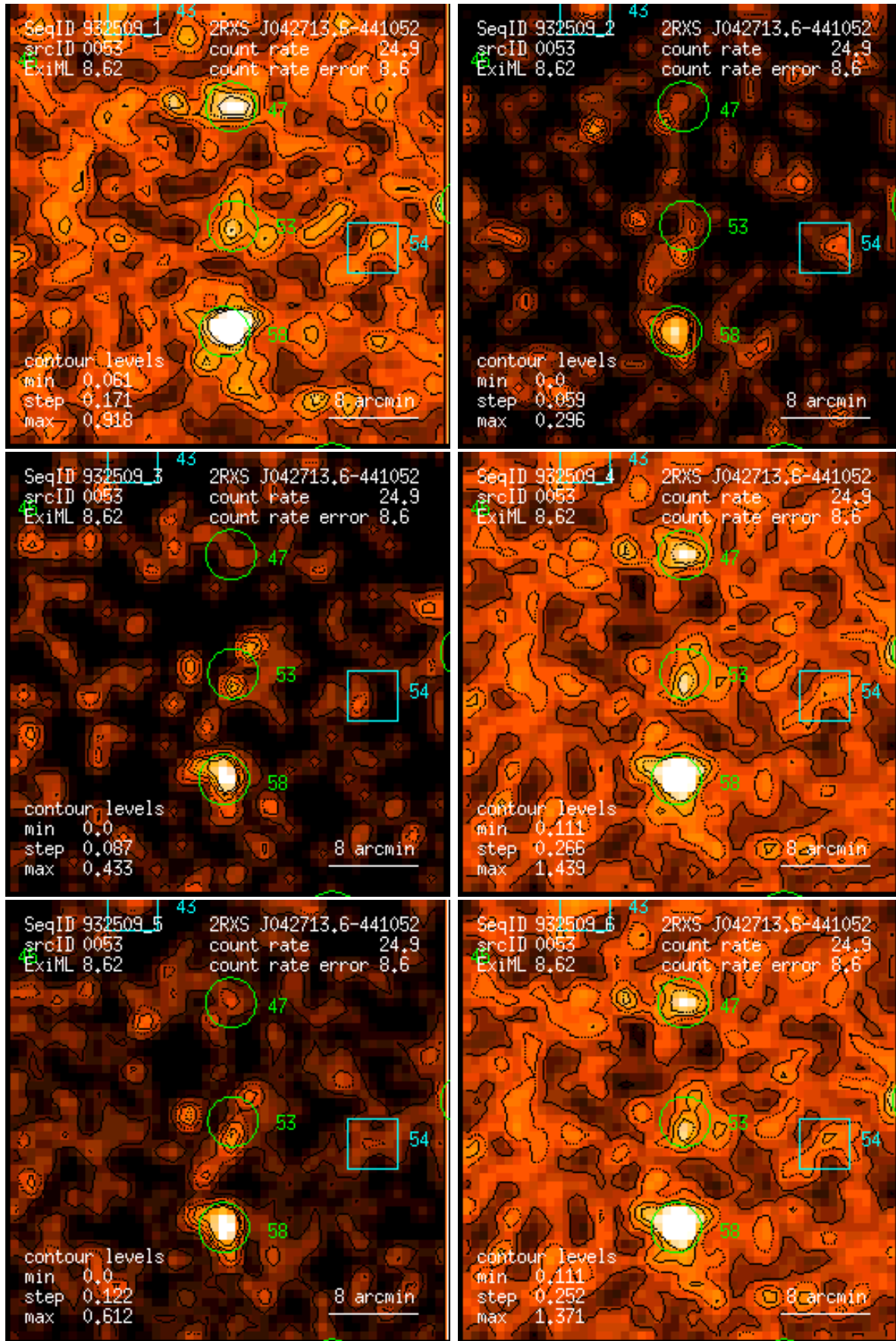
Figure 53: RASS 932509: detection 0053: band rate images, Gaussian filter: (1) PSPC channels 11 – 41, (2) 52 – 90, (3) 91 – 201, (4) 11 – 235, (5) 52 – 201, (6) 11 – 201. Broad band rates in counts/ks. Band rate contour levels in counts/ks/arcmin 2 .
