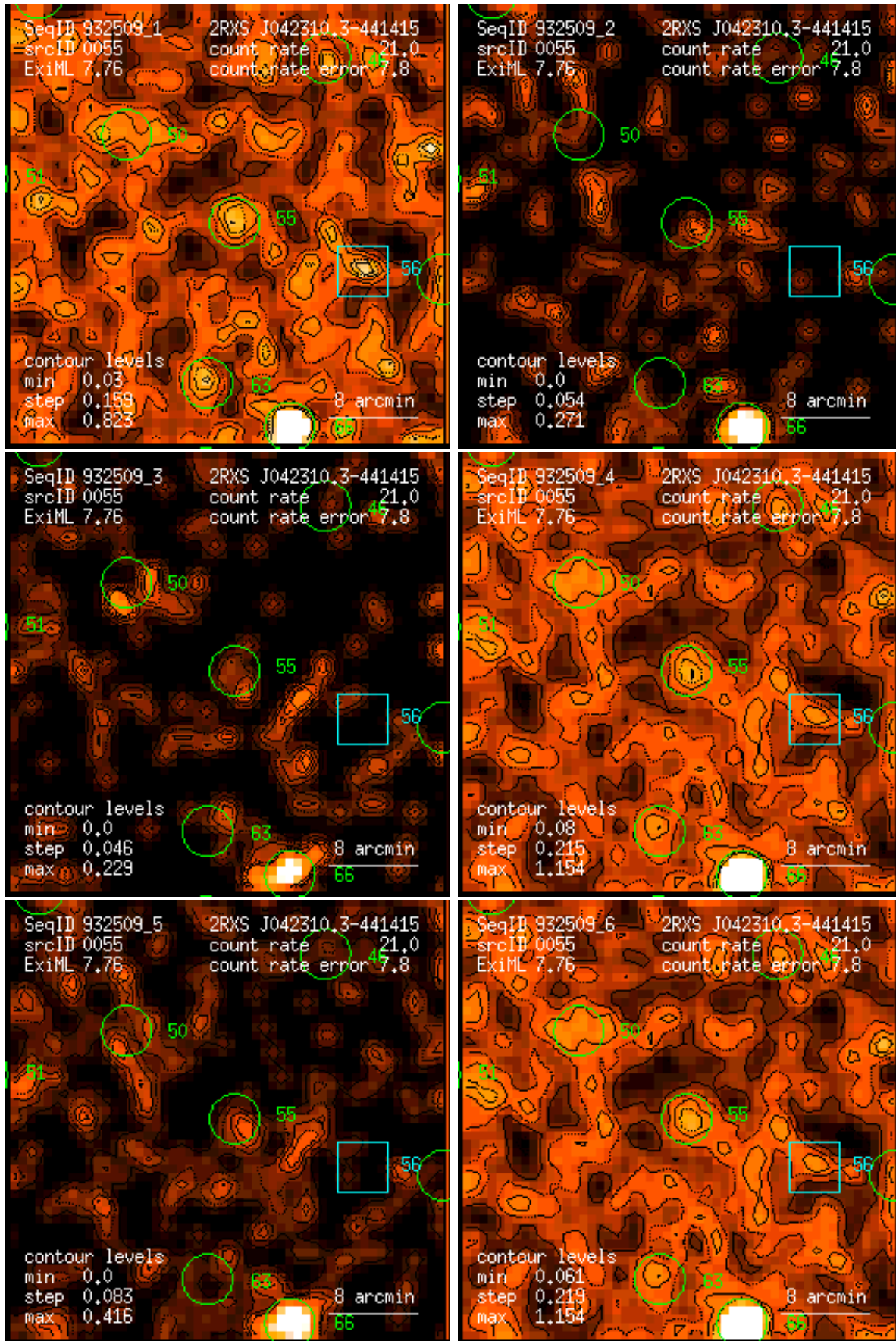
Figure 55: RASS 932509: detection 0055: band rate images, Gaussian filter: (1) PSPC channels 11 – 41, (2) 52 – 90, (3) 91 – 201, (4) 11 – 235, (5) 52 – 201, (6) 11 – 201. Broad band rates in counts/ks. Band rate contour levels in counts/ks/arcmin 2 .
