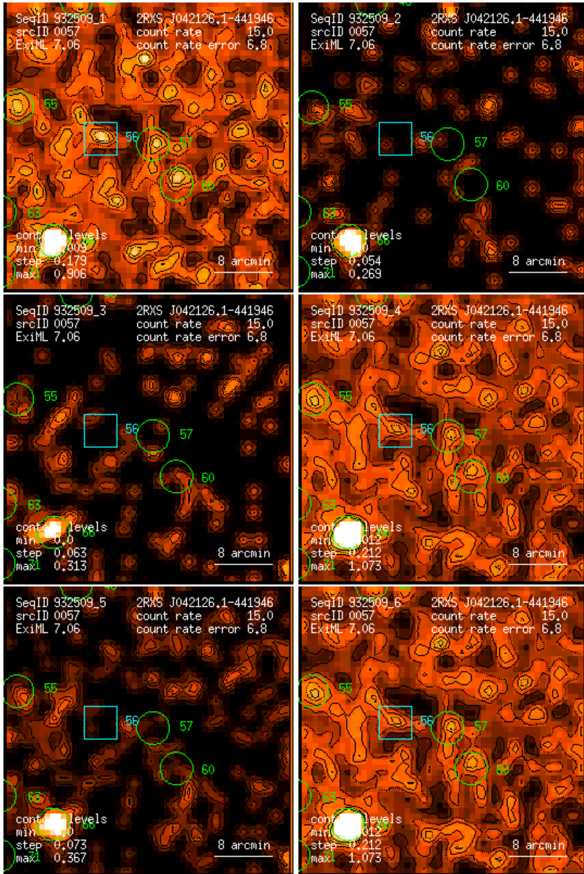
Figure 57: RASS 932509: detection 0057: band rate images, Gaussian filter: (1) PSPC channels 11 – 41, (2) 52 – 90, (3) 91 – 201, (4) 11 – 235, (5) 52 – 201, (6) 11 – 201. Broad band rates in counts/ks. Band rate contour levels in counts/ks/arcmin 2 .
