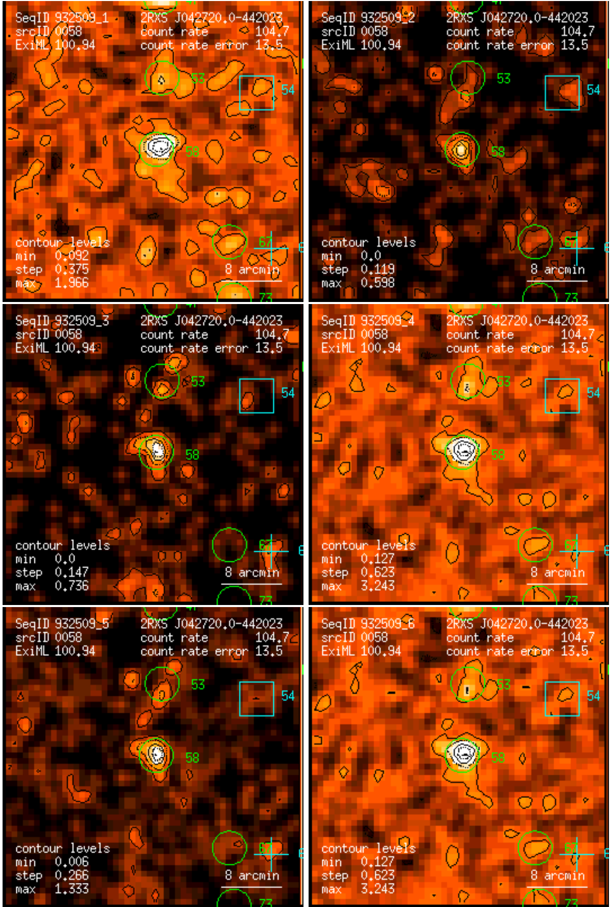
Figure 58: RASS 932509: detection 0058: band rate images, Gaussian filter: (1) PSPC channels 11 – 41, (2) 52 – 90, (3) 91 – 201, (4) 11 – 235, (5) 52 – 201, (6) 11 – 201. Broad band rates in counts/ks. Band rate contour levels in counts/ks/arcmin 2 .
