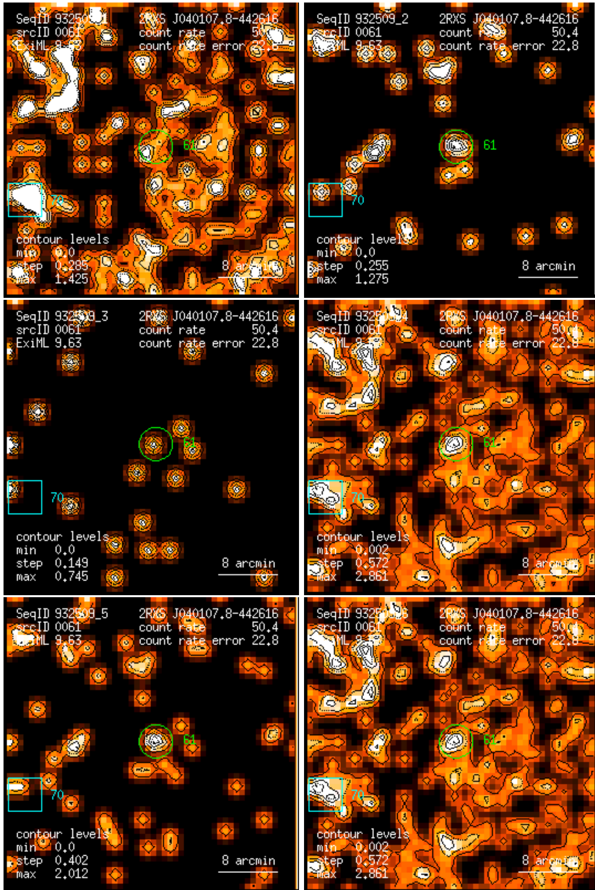
Figure 61: RASS 932509: detection 0061: band rate images, Gaussian filter: (1) PSPC channels 11 – 41, (2) 52 – 90, (3) 91 – 201, (4) 11 – 235, (5) 52 – 201, (6) 11 – 201. Broad band rates in counts/ks. Band rate contour levels in counts/ks/arcmin 2 .
