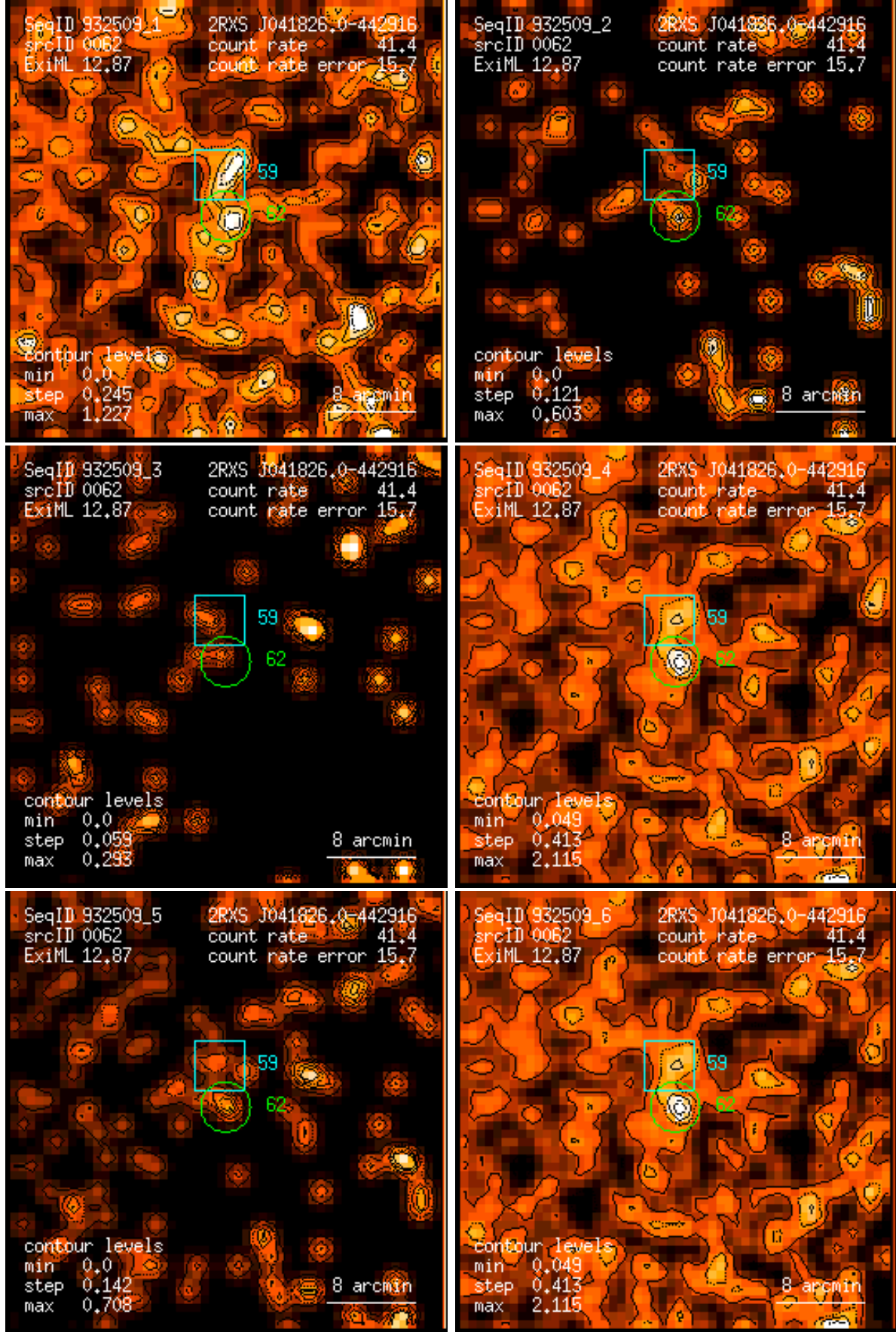
Figure 62: RASS 932509: detection 0062: band rate images, Gaussian filter: (1) PSPC channels 11 – 41, (2) 52 – 90, (3) 91 – 201, (4) 11 – 235, (5) 52 – 201, (6) 11 – 201. Broad band rates in counts/ks. Band rate contour levels in counts/ks/arcmin 2 .
