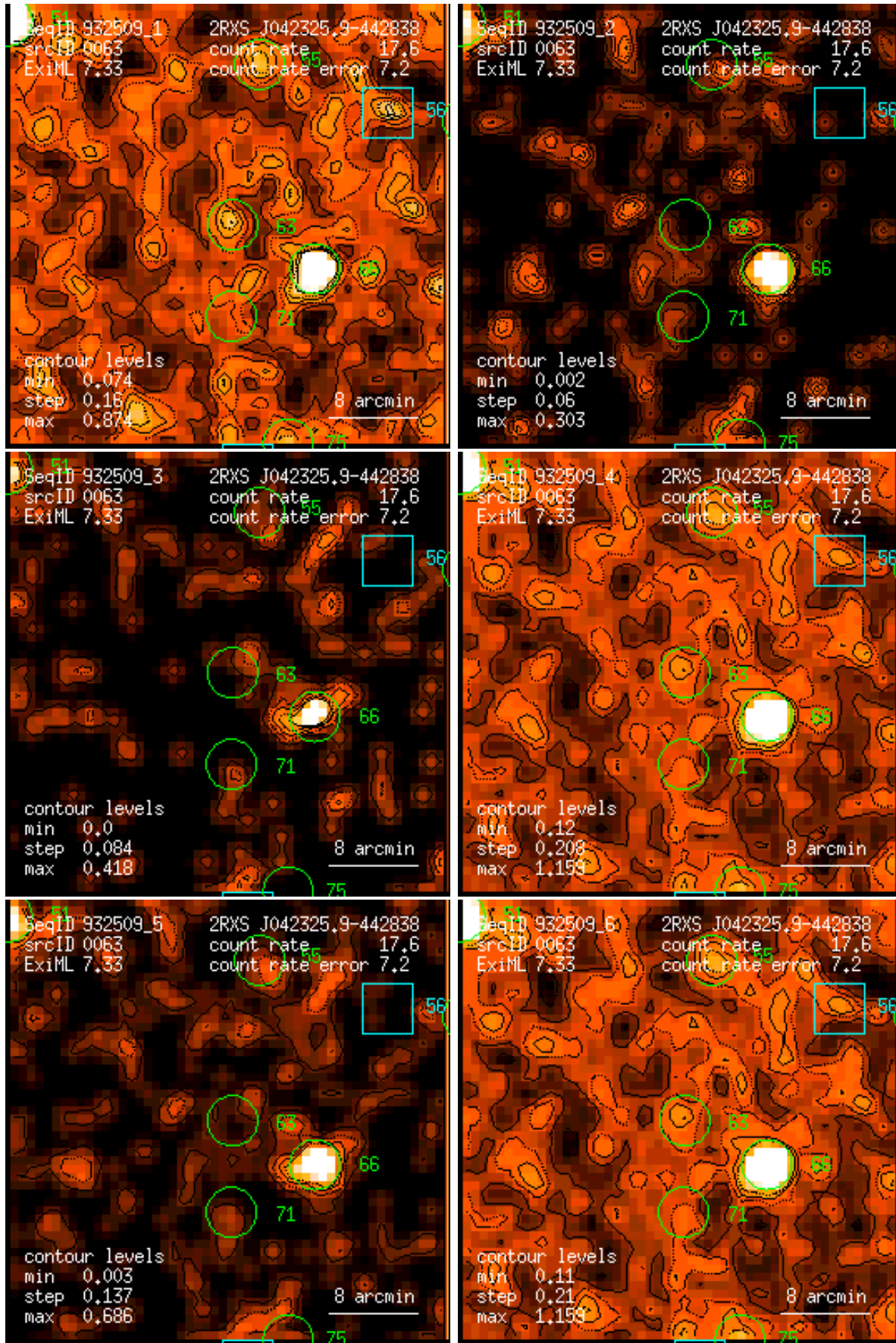
Figure 63: RASS 932509: detection 0063: band rate images, Gaussian filter: (1) PSPC channels 11 – 41, (2) 52 – 90, (3) 91 – 201, (4) 11 – 235, (5) 52 – 201, (6) 11 – 201. Broad band rates in counts/ks. Band rate contour levels in counts/ks/arcmin 2 .
