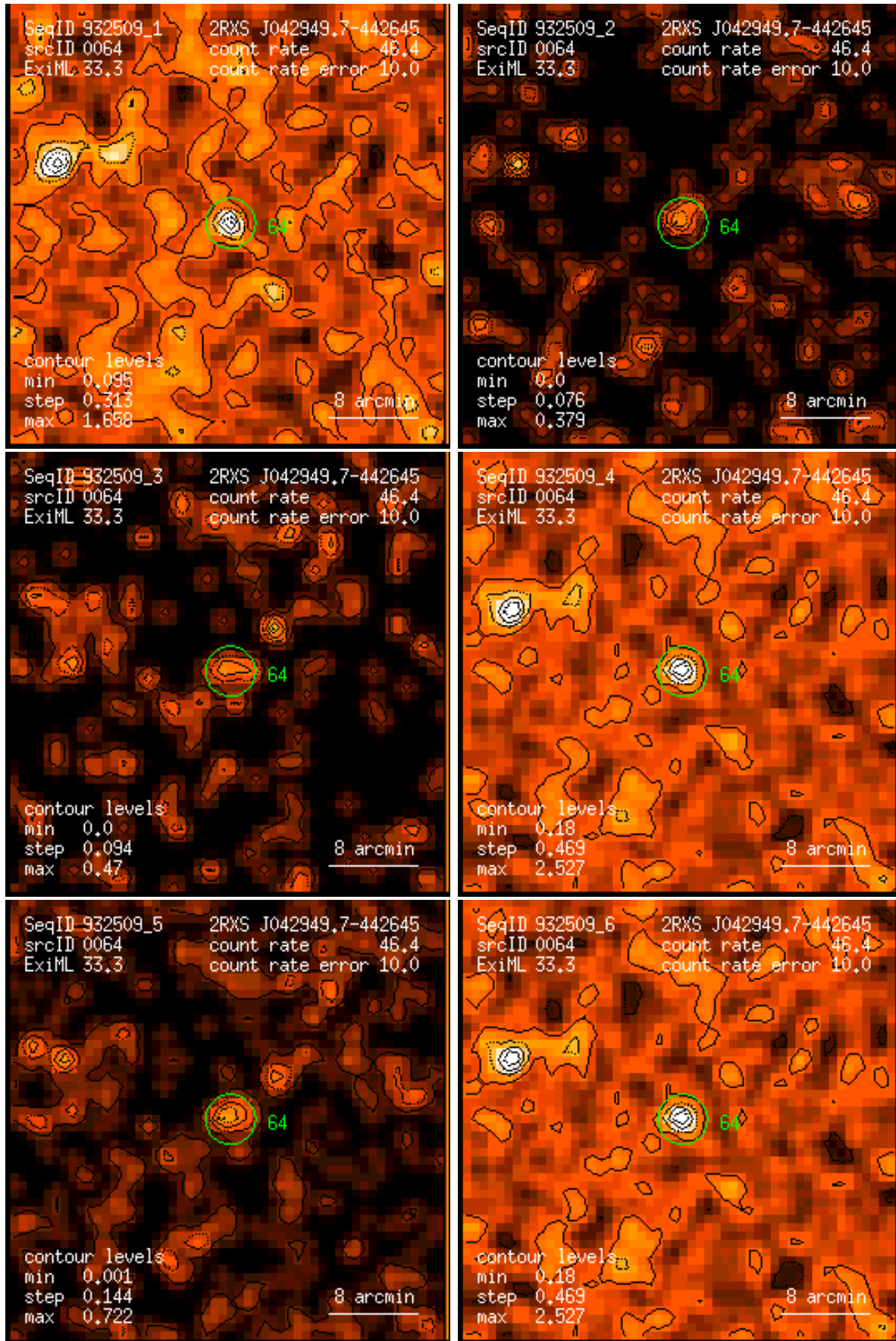
Figure 64: RASS 932509: detection 0064: band rate images, Gaussian filter: (1) PSPC channels 11 – 41, (2) 52 – 90, (3) 91 – 201, (4) 11 – 235, (5) 52 – 201, (6) 11 – 201. Broad band rates in counts/ks. Band rate contour levels in counts/ks/arcmin 2 .
