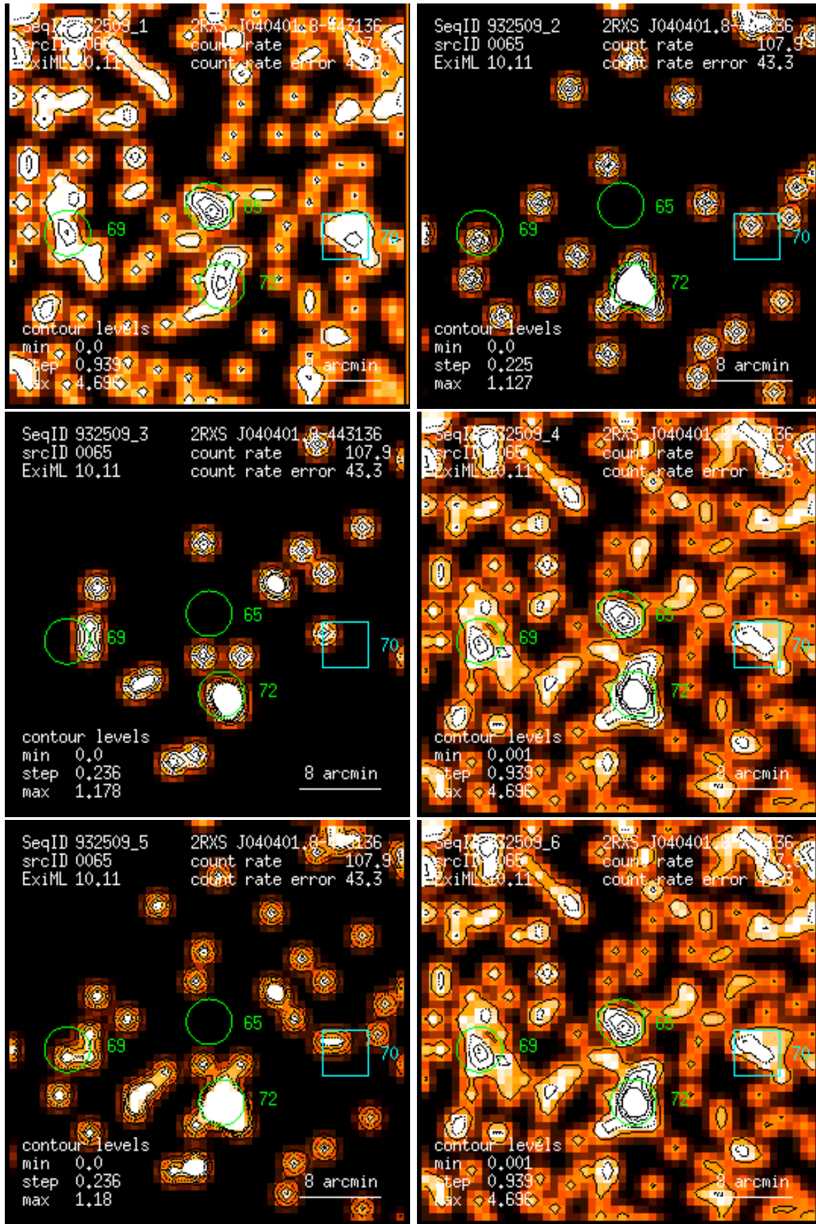
Figure 65: RASS 932509: detection 0065: band rate images, Gaussian filter: (1) PSPC channels 11 – 41, (2) 52 – 90, (3) 91 – 201, (4) 11 – 235, (5) 52 – 201, (6) 11 – 201. Broad band rates in counts/ks. Band rate contour levels in counts/ks/arcmin 2 .
