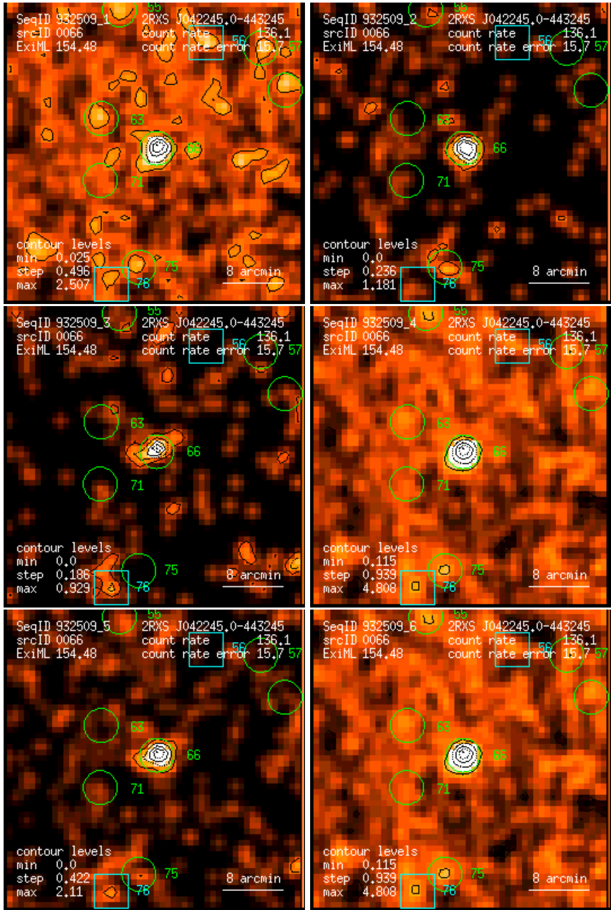
Figure 66: RASS 932509: detection 0066: band rate images, Gaussian filter: (1) PSPC channels 11 – 41, (2) 52 – 90, (3) 91 – 201, (4) 11 – 235, (5) 52 – 201, (6) 11 – 201. Broad band rates in counts/ks. Band rate contour levels in counts/ks/arcmin 2 .
