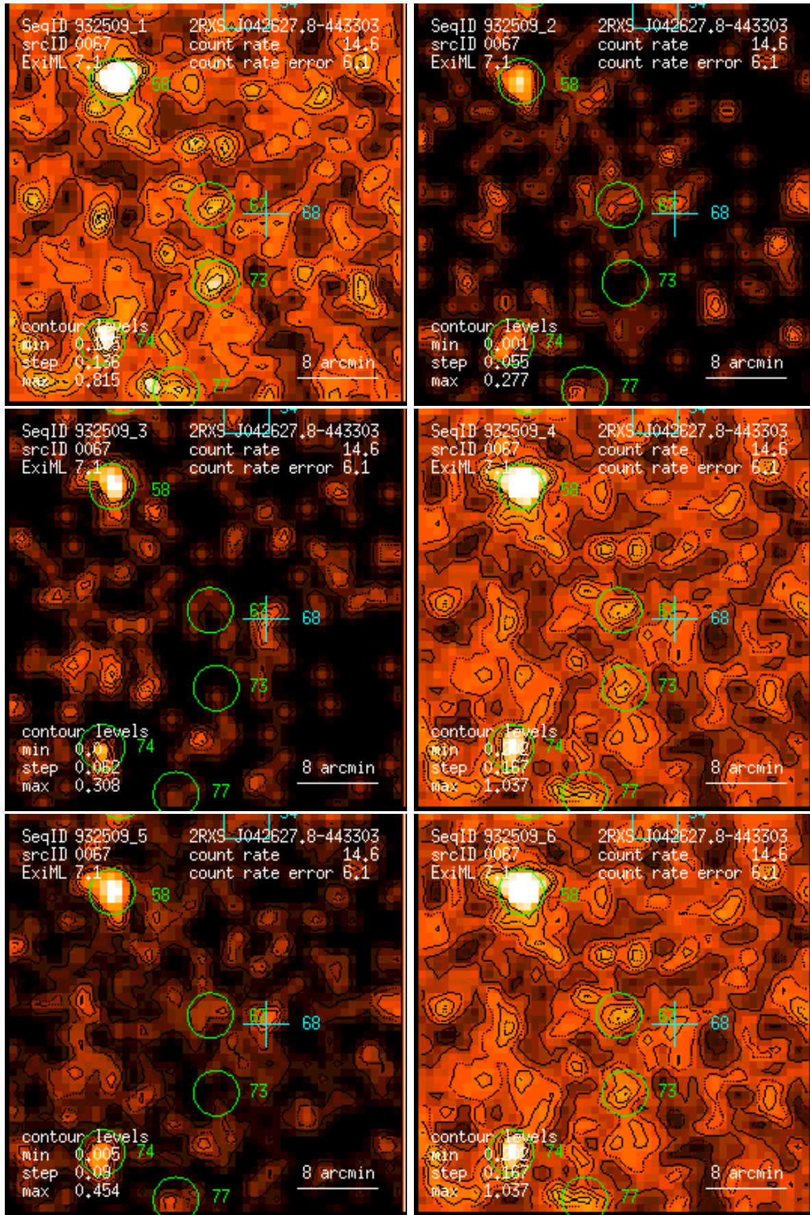
Figure 67: RASS 932509: detection 0067: band rate images, Gaussian filter: (1) PSPC channels 11 – 41, (2) 52 – 90, (3) 91 – 201, (4) 11 – 235, (5) 52 – 201, (6) 11 – 201. Broad band rates in counts/ks. Band rate contour levels in counts/ks/arcmin 2 .
