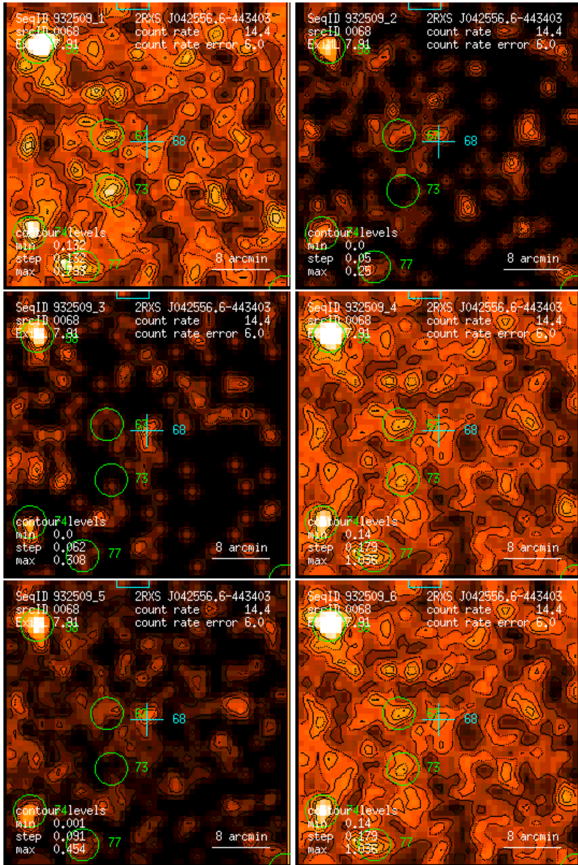
Figure 68: RASS 932509: detection 0068: band rate images, Gaussian filter: (1) PSPC channels 11 – 41, (2) 52 – 90, (3) 91 – 201, (4) 11 – 235, (5) 52 – 201, (6) 11 – 201. Broad band rates in counts/ks. Band rate contour levels in counts/ks/arcmin 2 .
