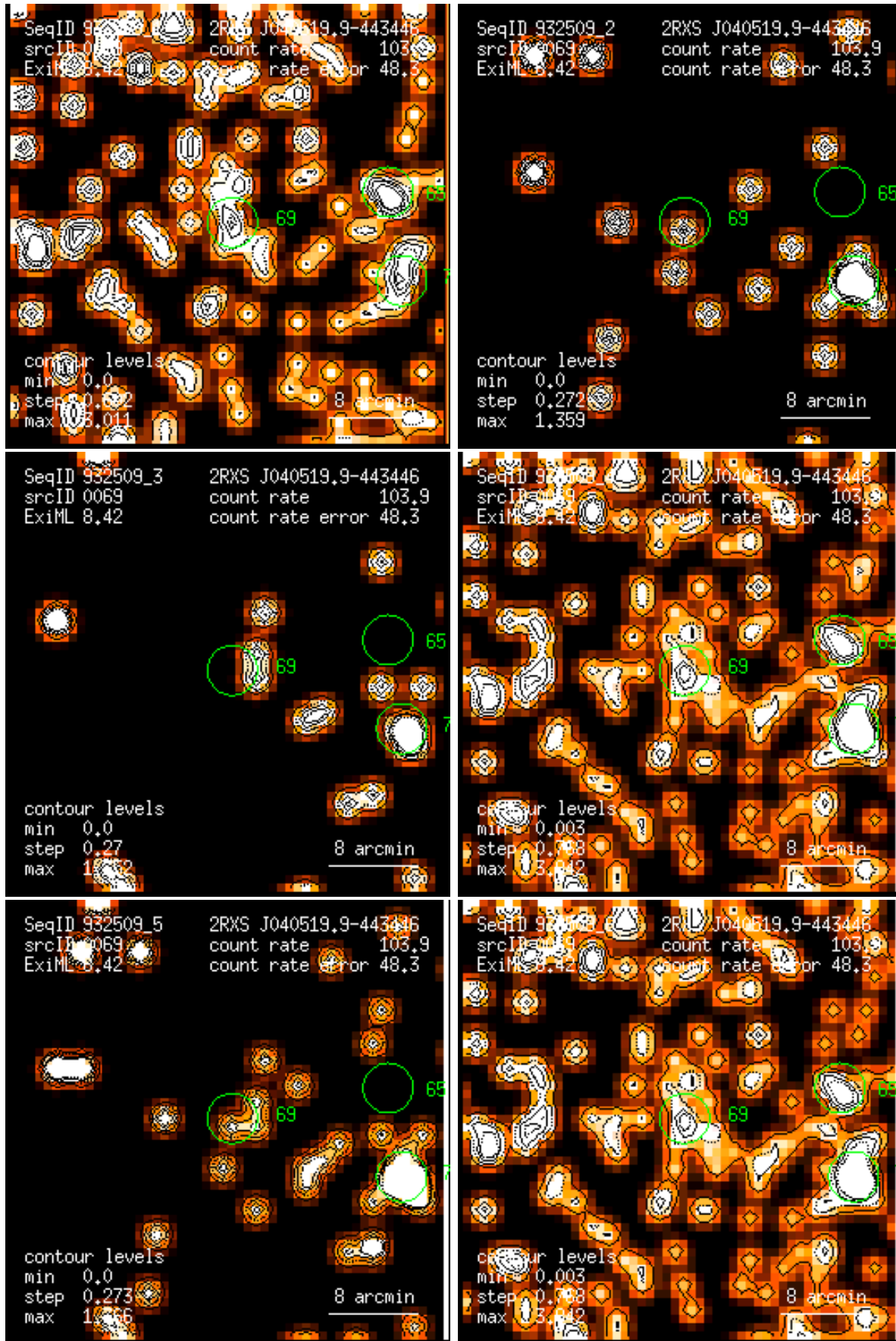
Figure 69: RASS 932509: detection 0069: band rate images, Gaussian filter: (1) PSPC channels 11 – 41, (2) 52 – 90, (3) 91 – 201, (4) 11 – 235, (5) 52 – 201, (6) 11 – 201. Broad band rates in counts/ks. Band rate contour levels in counts/ks/arcmin 2 .
