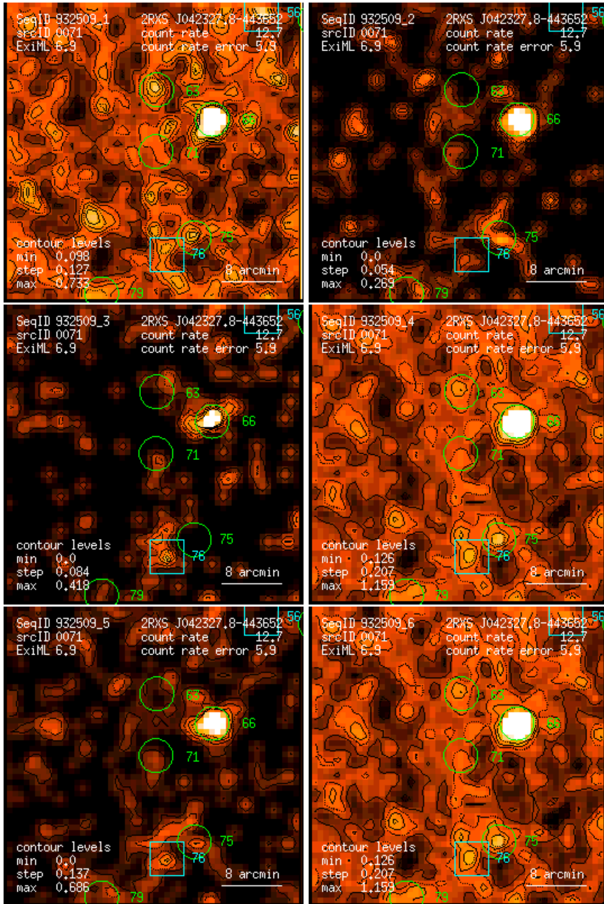
Figure 71: RASS 932509: detection 0071: band rate images, Gaussian filter: (1) PSPC channels 11 – 41, (2) 52 – 90, (3) 91 – 201, (4) 11 – 235, (5) 52 – 201, (6) 11 – 201. Broad band rates in counts/ks. Band rate contour levels in counts/ks/arcmin 2 .
