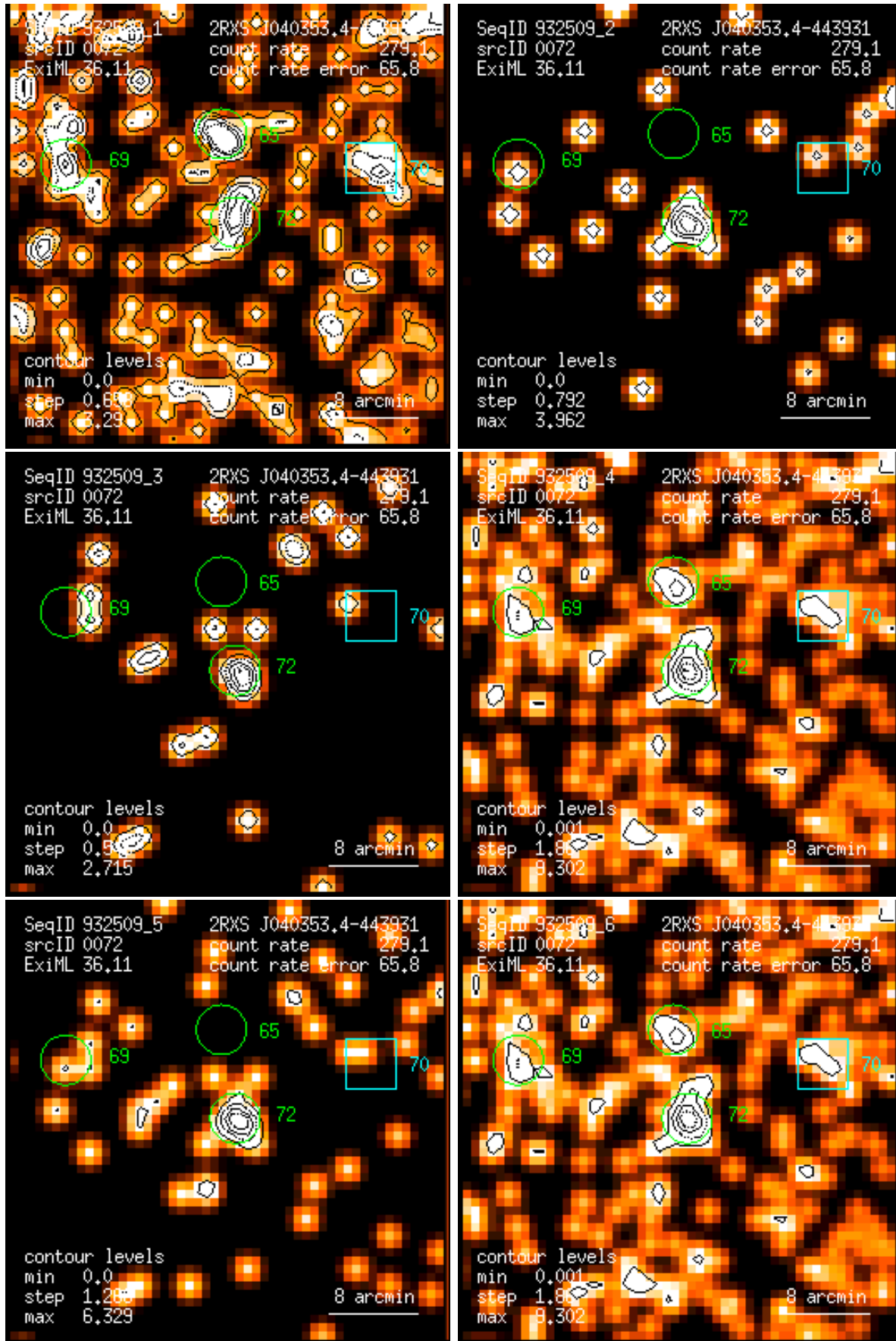
Figure 72: RASS 932509: detection 0072: band rate images, Gaussian filter: (1) PSPC channels 11 – 41, (2) 52 – 90, (3) 91 – 201, (4) 11 – 235, (5) 52 – 201, (6) 11 – 201. Broad band rates in counts/ks. Band rate contour levels in counts/ks/arcmin 2 .
