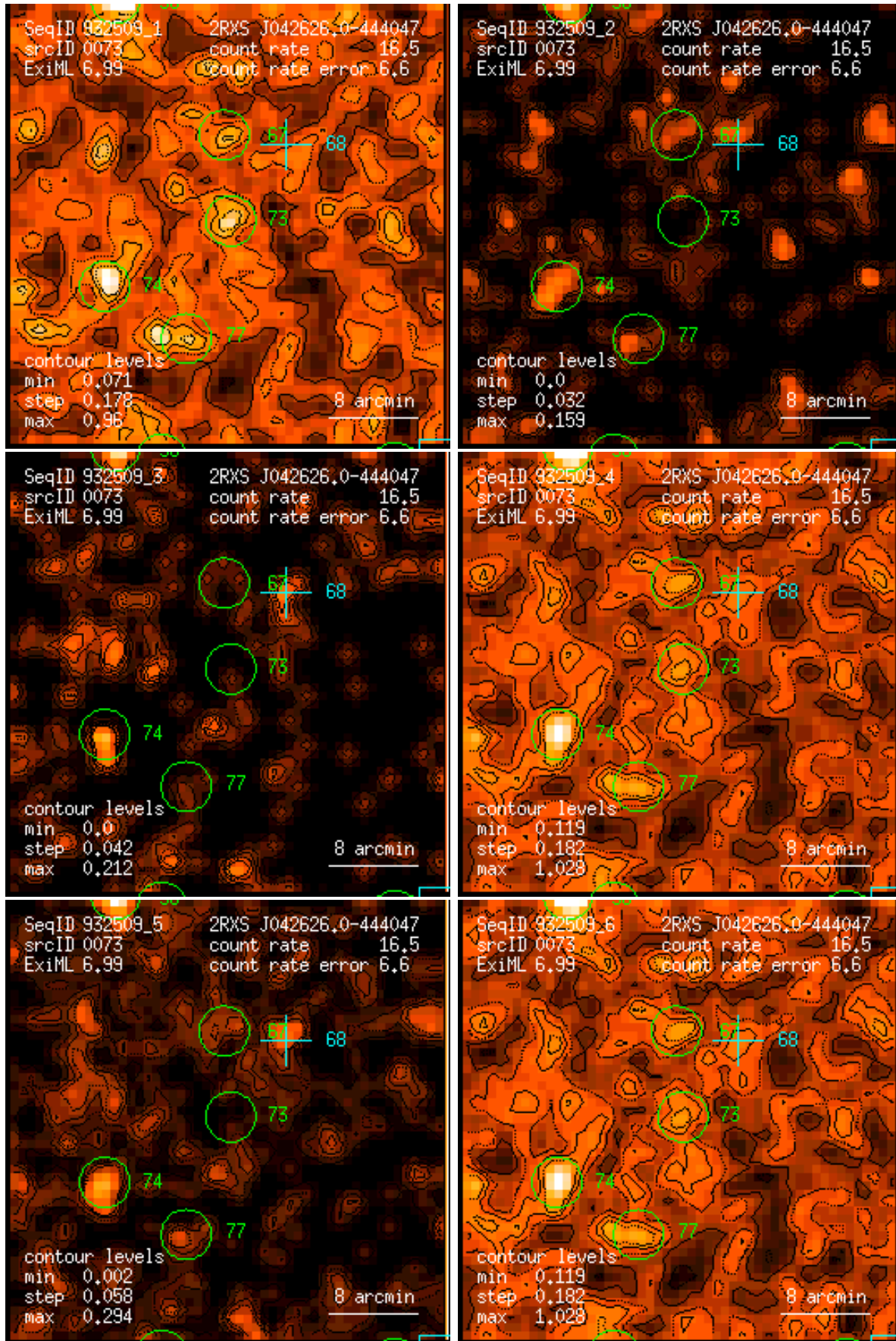
Figure 73: RASS 932509: detection 0073: band rate images, Gaussian filter: (1) PSPC channels 11 – 41, (2) 52 – 90, (3) 91 – 201, (4) 11 – 235, (5) 52 – 201, (6) 11 – 201. Broad band rates in counts/ks. Band rate contour levels in counts/ks/arcmin 2 .
