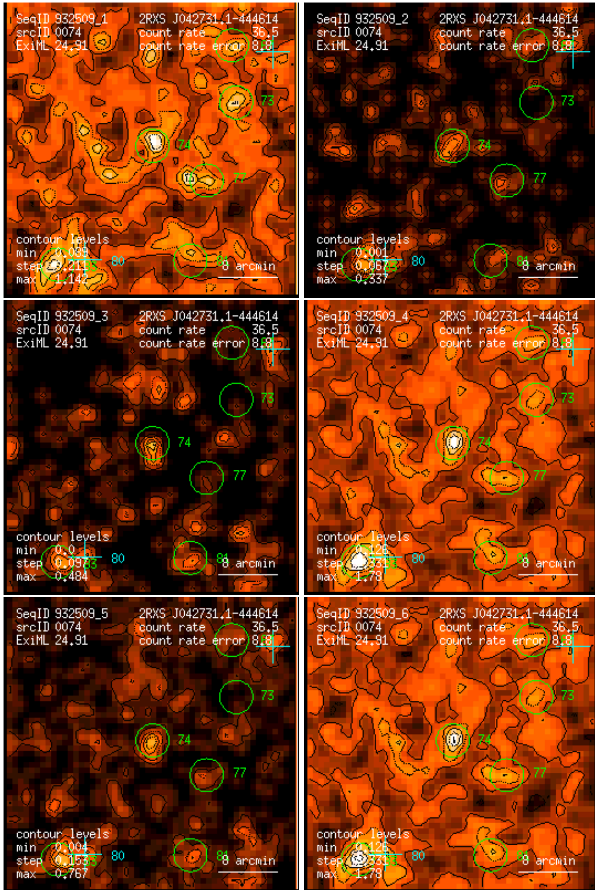
Figure 74: RASS 932509: detection 0074: band rate images, Gaussian filter: (1) PSPC channels 11 – 41, (2) 52 – 90, (3) 91 – 201, (4) 11 – 235, (5) 52 – 201, (6) 11 – 201. Broad band rates in counts/ks. Band rate contour levels in counts/ks/arcmin 2 .
