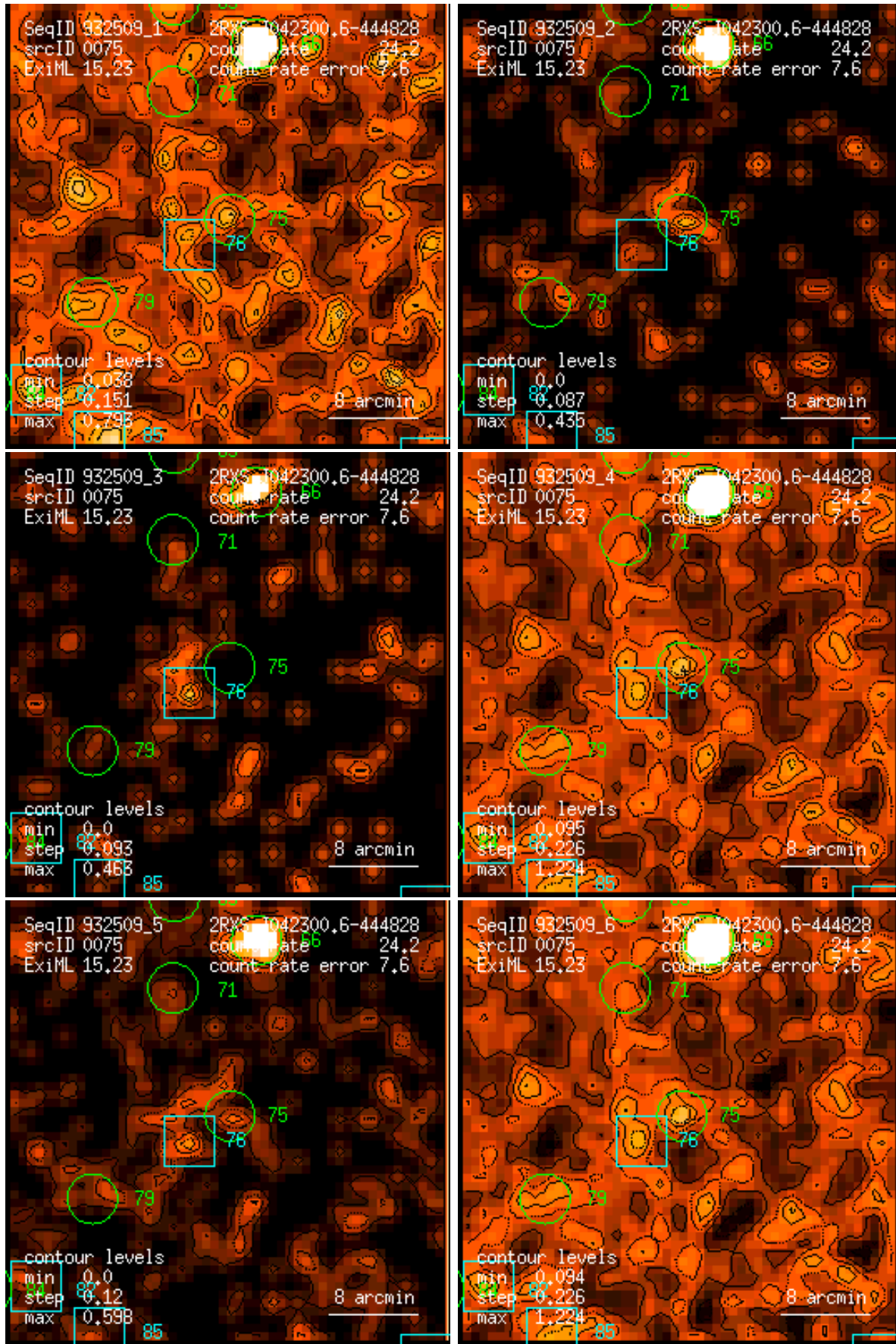
Figure 75: RASS 932509: detection 0075: band rate images, Gaussian filter: (1) PSPC channels 11 – 41, (2) 52 – 90, (3) 91 – 201, (4) 11 – 235, (5) 52 – 201, (6) 11 – 201. Broad band rates in counts/ks. Band rate contour levels in counts/ks/arcmin 2 .
